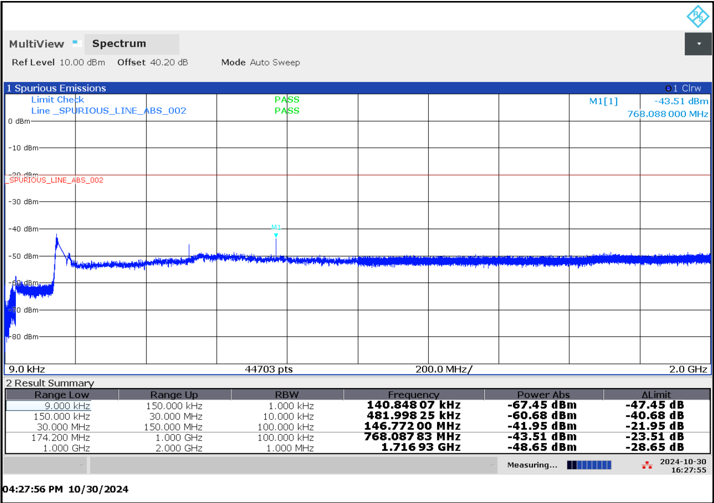
Plot 6-7: Conducted Spurious Emissions – 173.9875 MHz
