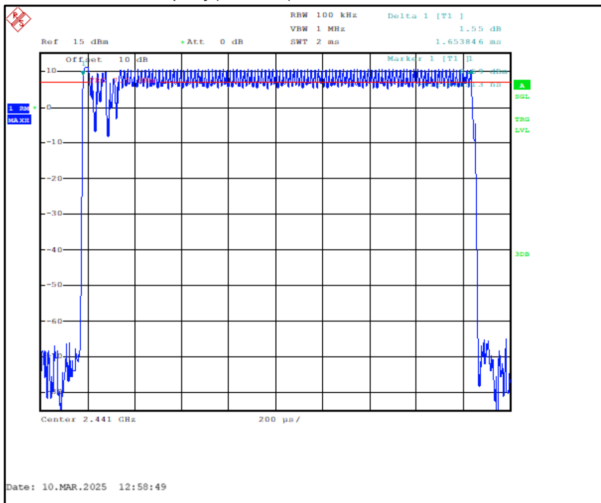
Plot 9-1: Time of Occupancy (Dwell Time)
