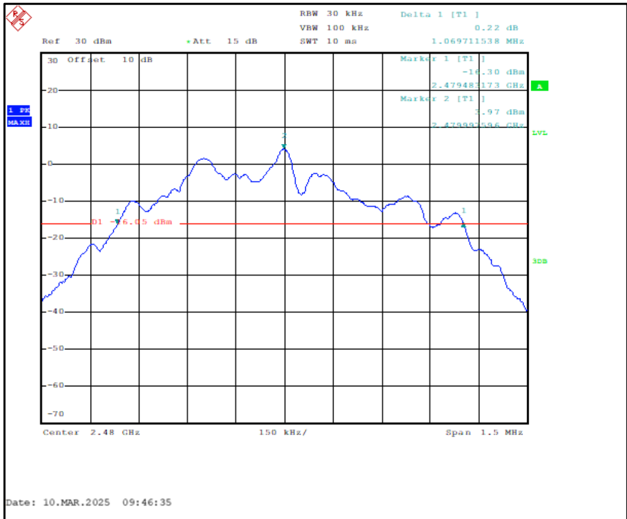
Plot 6-3: 20 dB Bandwidth – 2480 MHz – GFSK
