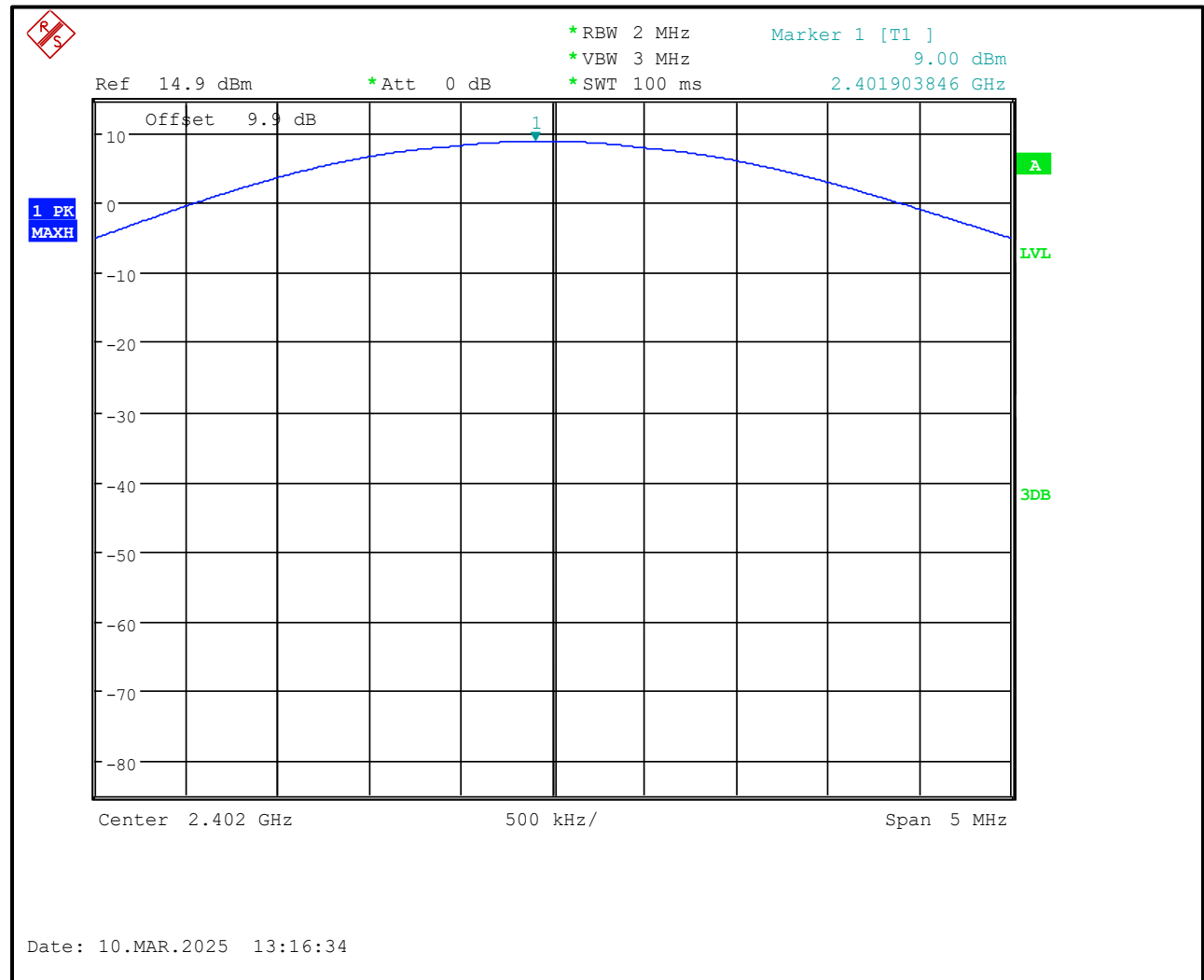
Plot 3-1: Peak Power; 2402 MHz
