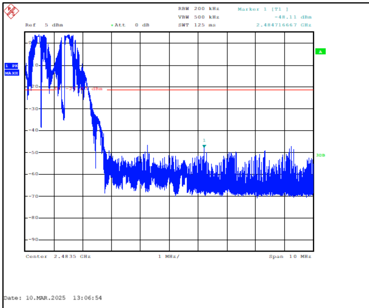
Plot 4-4: Upper Band Edge – Peak – GFSK
