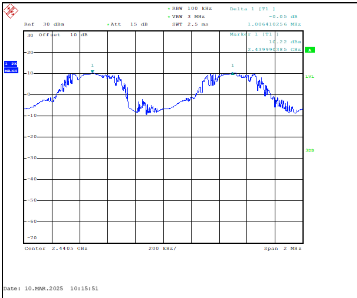
Plot 7-1: Carrier Frequency Separation
