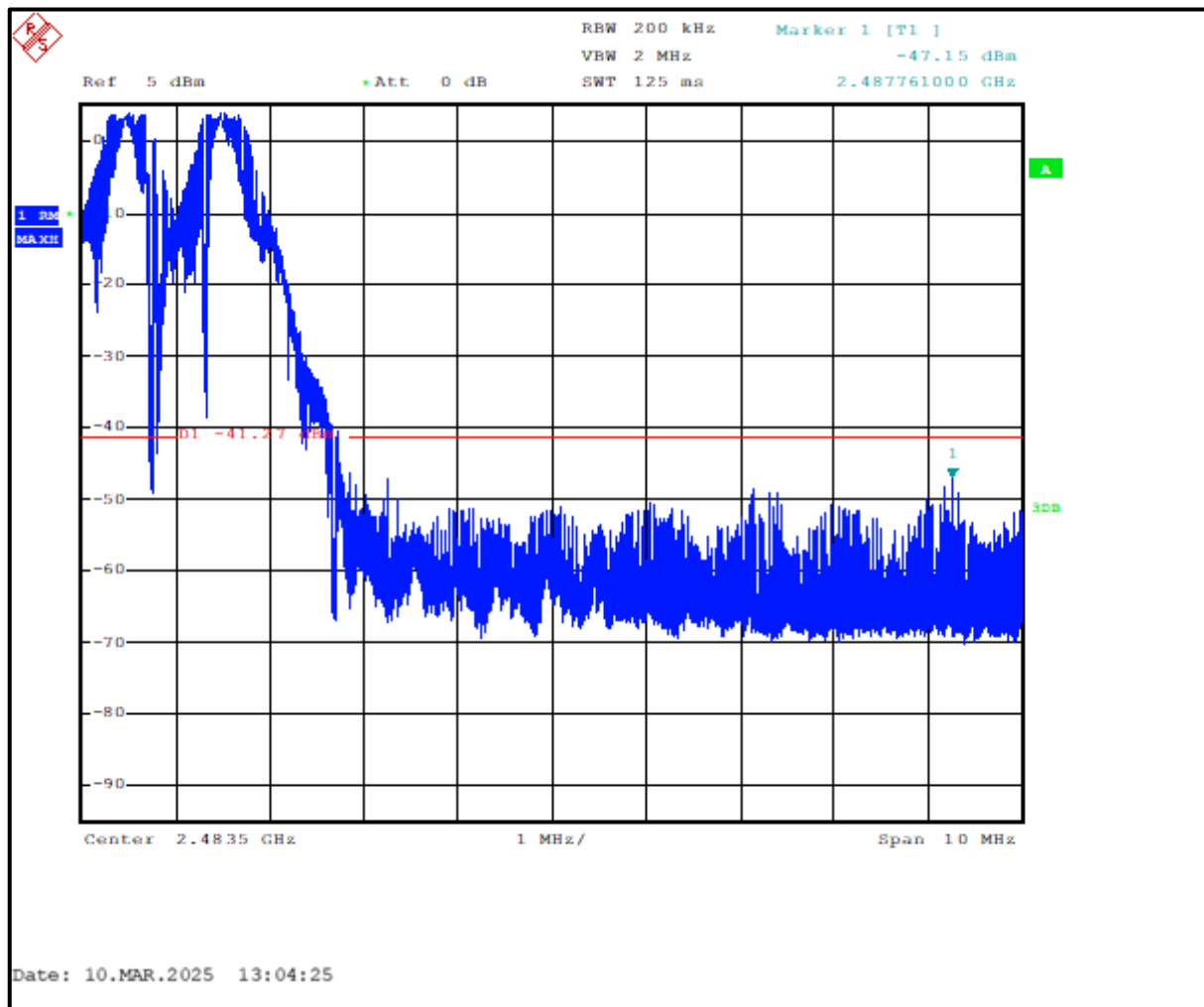
Plot 4-3: Upper Band Edge – Average
