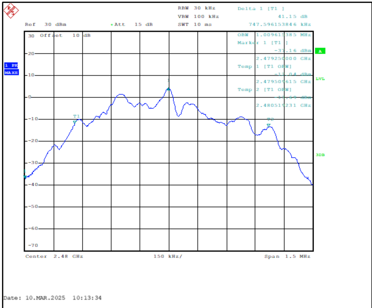
Plot 6-6: 99% Bandwidth – 2480 MHz – GFSK
