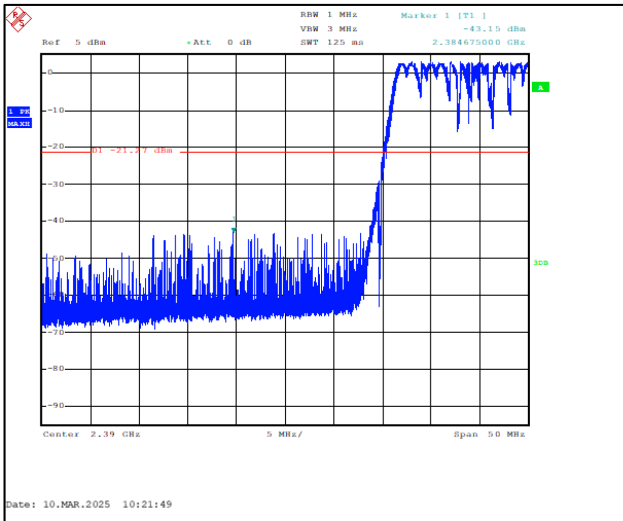
Plot 4-2: Lower Band Edge – Peak
