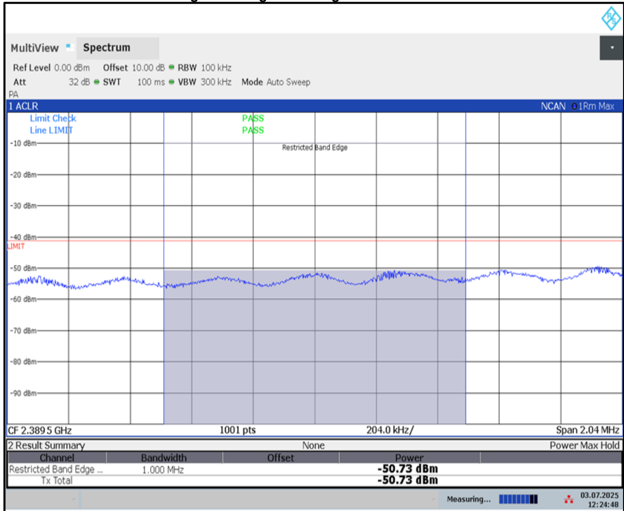
Plot 4-5: Lower Band Edge – Average – 802.11g
