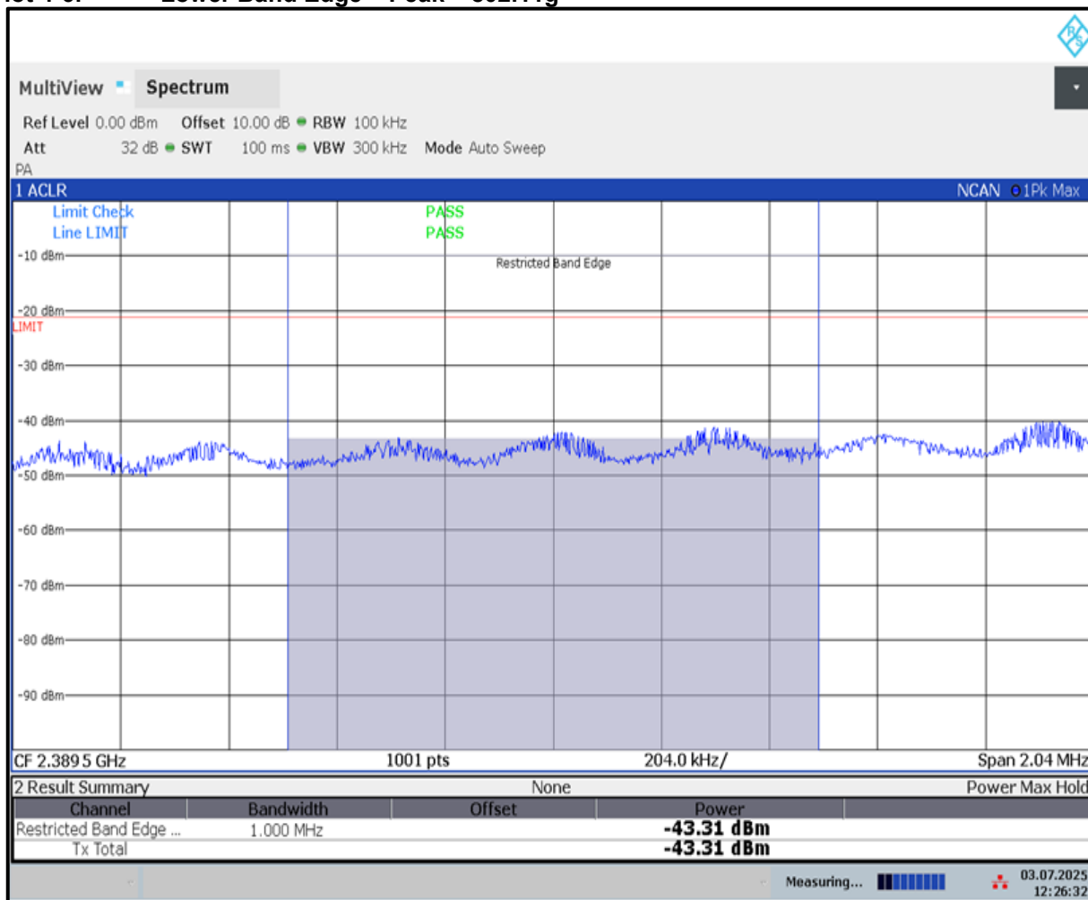
Plot 4-6: Lower Band Edge – Peak – 802.11g
