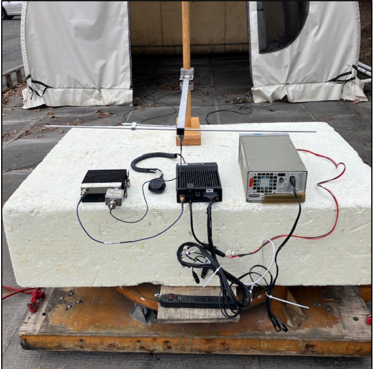
Photograph 2: Radiated Emissions – Back View (Below 1 GHz)
