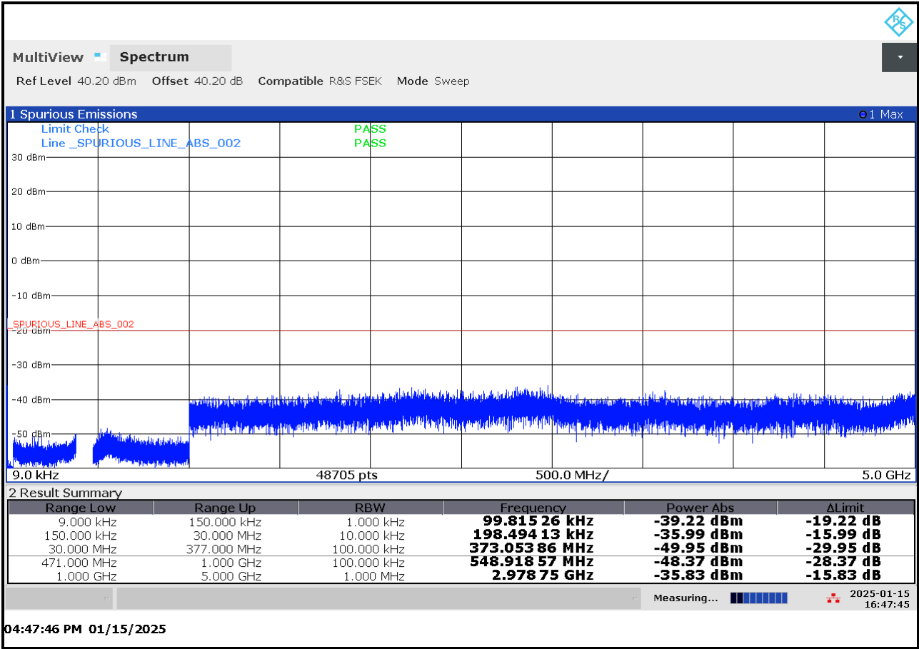
Plot 5-3: Conducted Antenna Spurious Emissions - 469.9875 MHz
