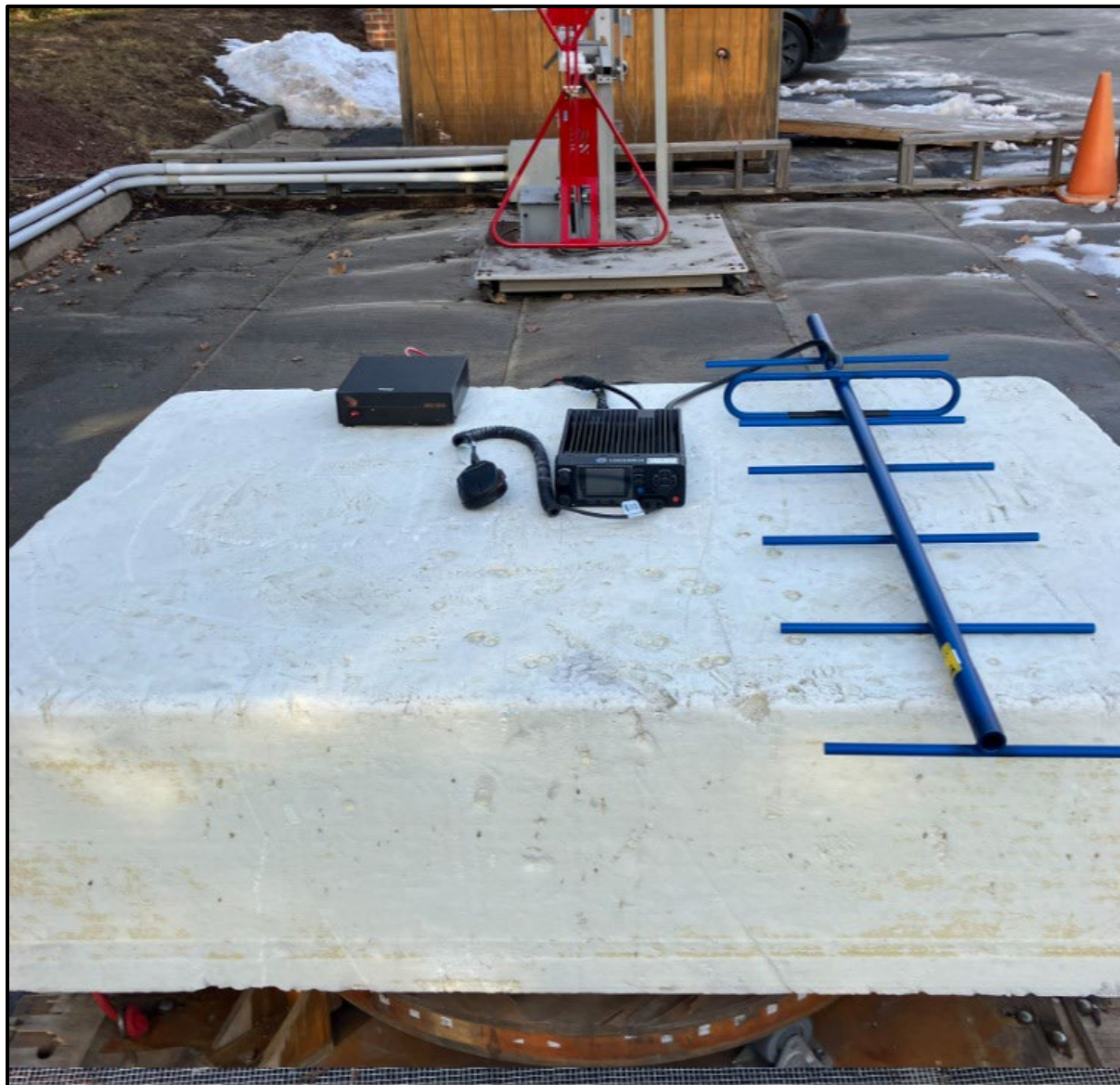
Photograph 1: Radiated Emissions (Spurious/Harmonics) (<1 GHz) - Front View
