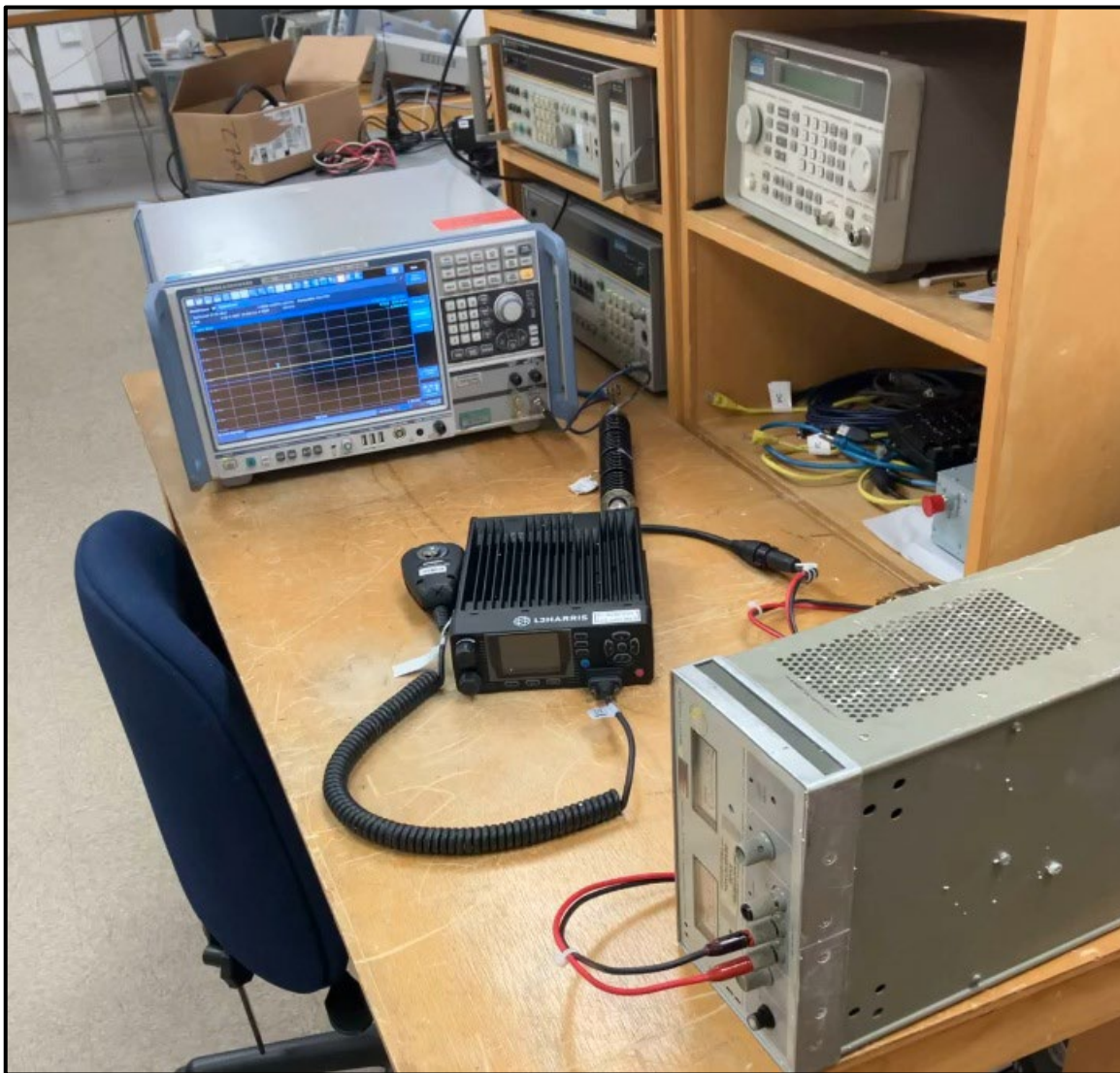
Photograph 5: Conducted Testing
