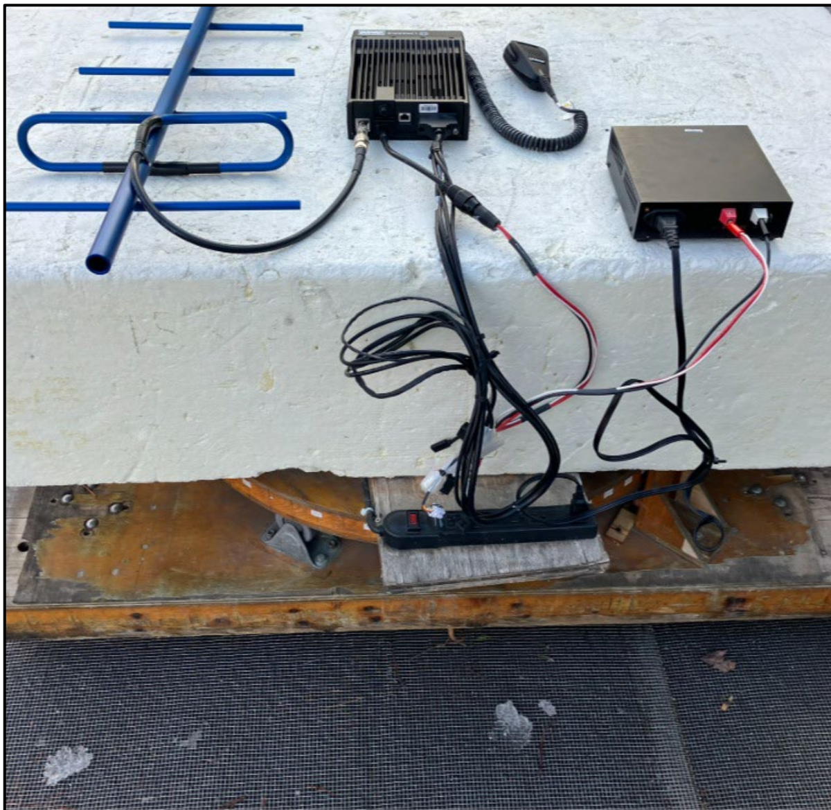
Photograph 2: Radiated Emissions (Spurious/Harmonics) (<1 GHz) – Back View
