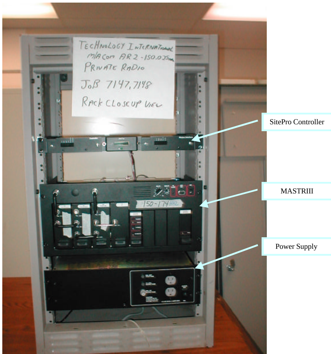
Figure 1. EUT Photograph (Front)
