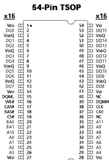
PIN ASSIGNMENT (Top View)
