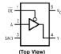
Connection Diagram
