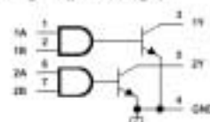
logic diagram (positive logic)
