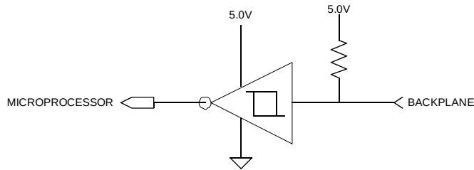
Figure 5 - Input Circuits U22A thru F, U29D and U32B
