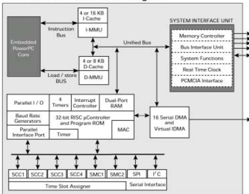
MPC860 Processor Block Diagram
