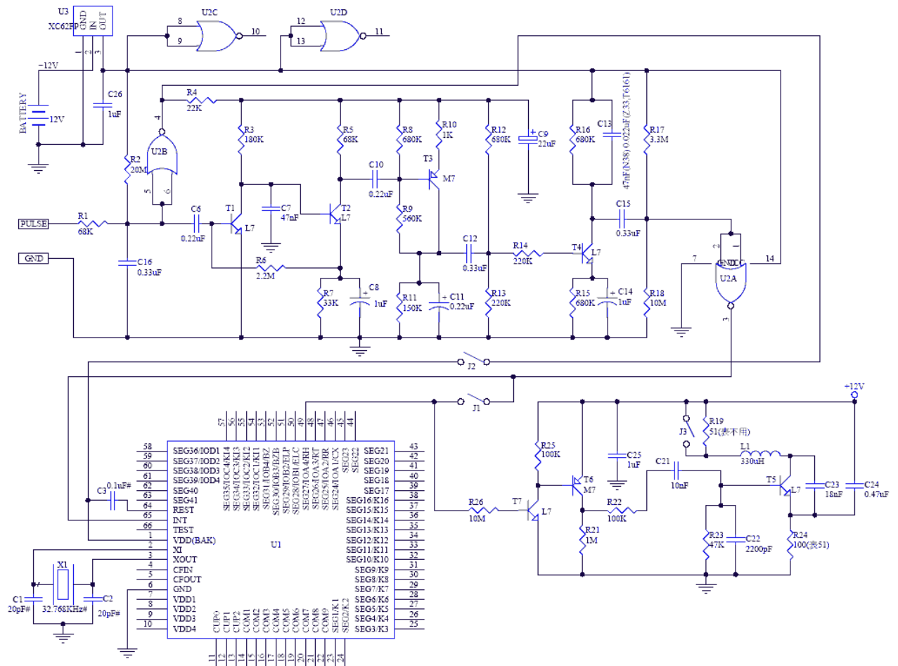
Figure 4.1 System Schematics
