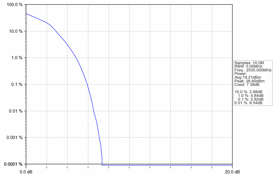
Band7_5MHz_16QAM_MCH_2535.000MHz_RB_25_0_NTNV
