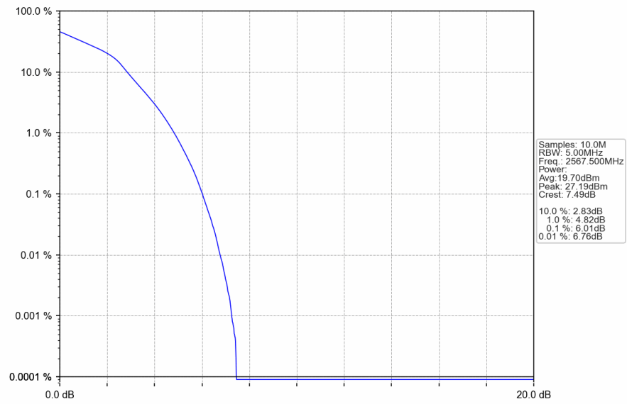
Band7_5MHz_16QAM_HCH_2567.500MHz_RB_25_0_NTNV
