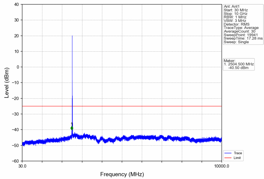
Band7_10MHz_16QAM_MCH_2535MHz_RB_1_0_NTNV
