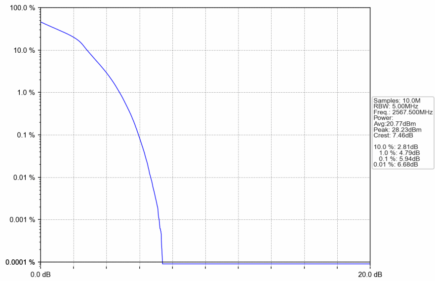
Band7_5MHz_16QAM_HCH_2567.500MHz_RB_25_0_NTNV
