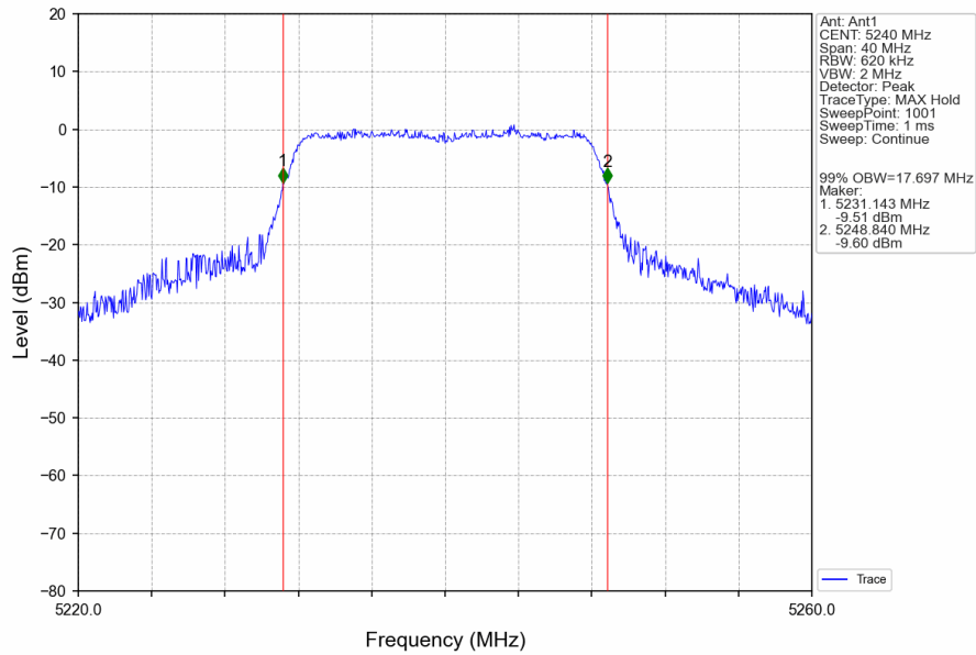
802.11a_HCH_5240MHz_Ant1_NTNV
