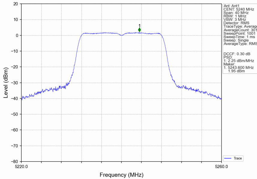
802.11a_HCH_5240MHz_Ant1_NTNV
