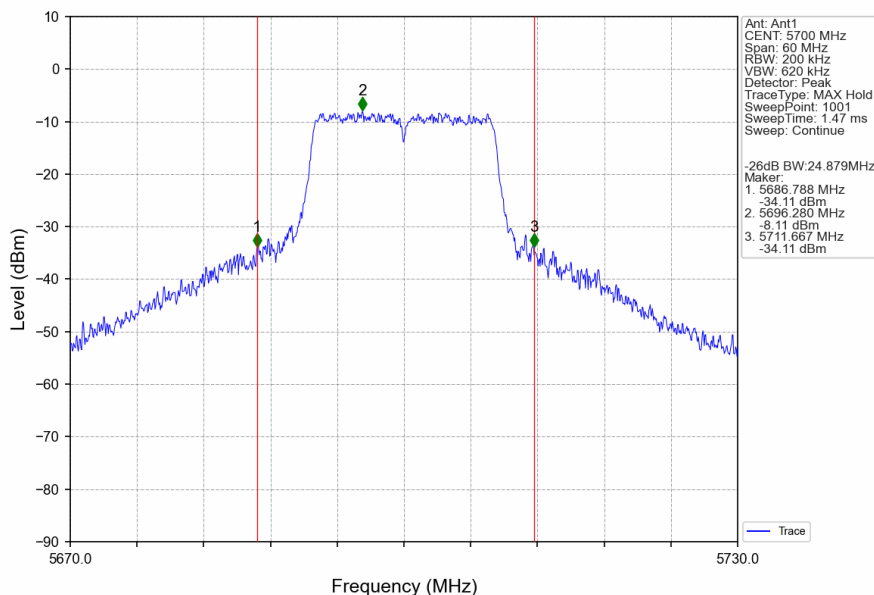
802.11a_HCH_5700MHz_Ant1_NTNV
