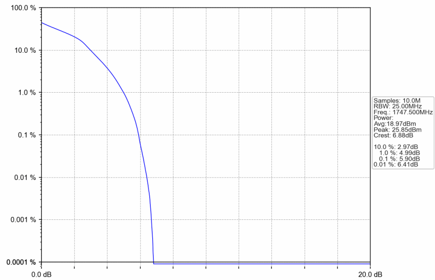
Band4_15MHz_16QAM_HCH_1747.5MHz_RB_75_0_NTNV
