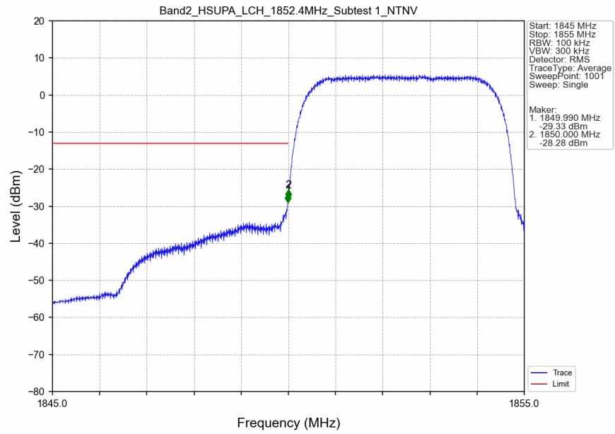
Band2_HSUPA_LCH_1852.4MHz_Subtest 1_NTNV
