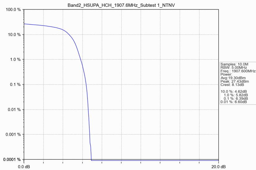
Band2_HSUPA_HCH_1907.6MHz_Subtest 1_NTNV
