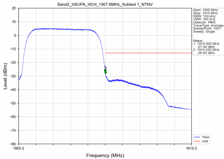
Band2_HSUPA_HCH_1907.6MHz_Subtest 1_NTNV
