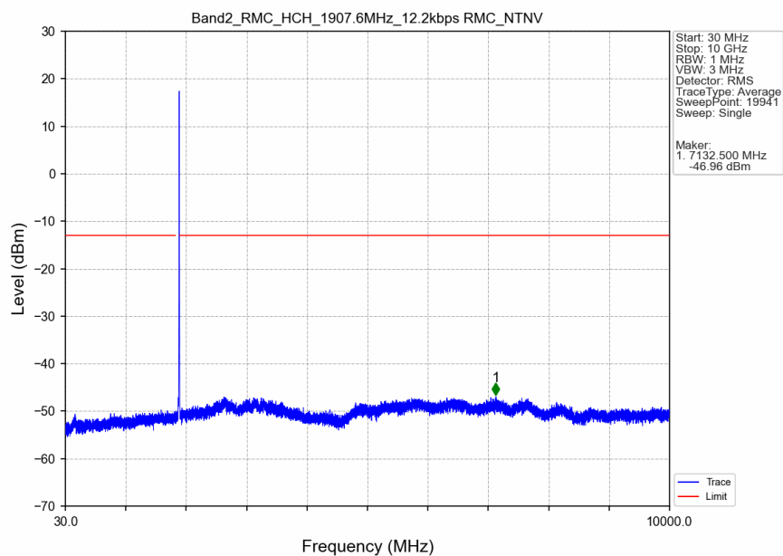
Band2_RMC_HCH_1907.6MHz_12.2kbps RMC_NTNV
