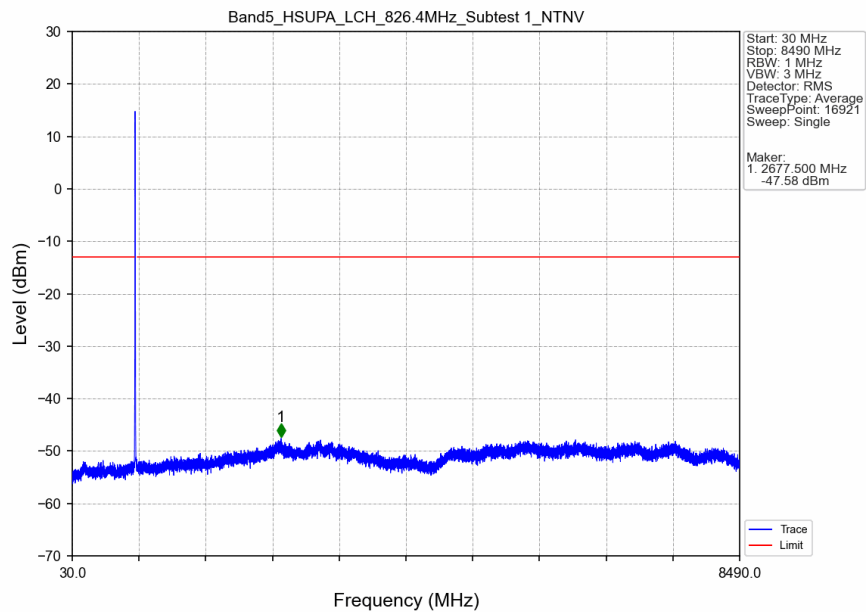
Band5_HSUPA_LCH_826.4MHz_Subtest 1_NTNV
