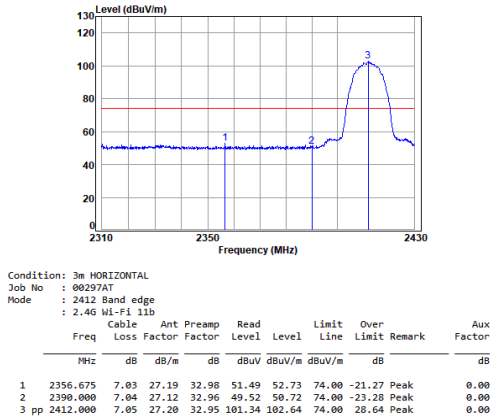
11b_TX_CH_01_Horizontal-Peak
