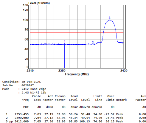
11b_TX_CH_01_Vertical-Peak
