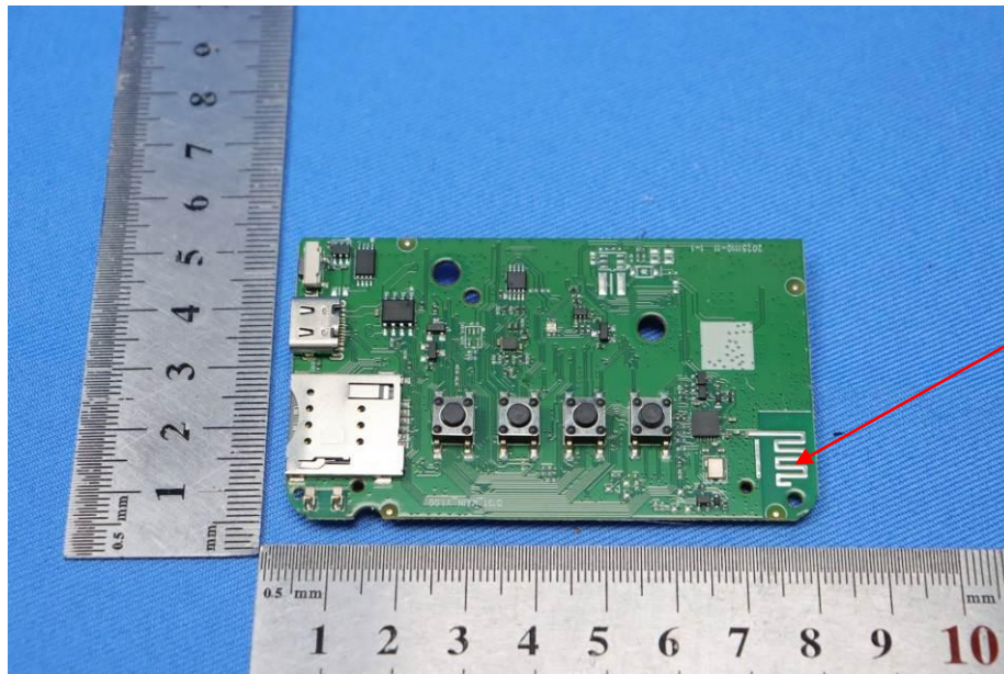
Wi-Fi antenna
