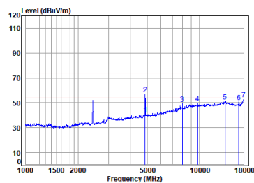
11g_TX_CH_06_Vertical
