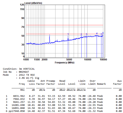
11g_TX_CH_01_Vertical
