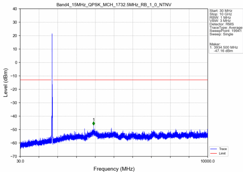
Band4_15MHz_QPSK_MCH_1732.5MHz_RB_1_0_NTNV
