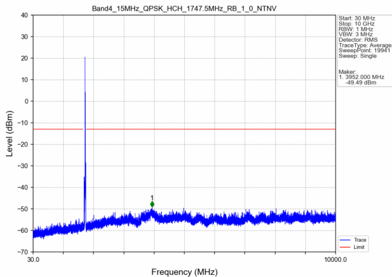
Band4_15MHz_QPSK_HCH_1747.5MHz_RB_1_0_NTNV
