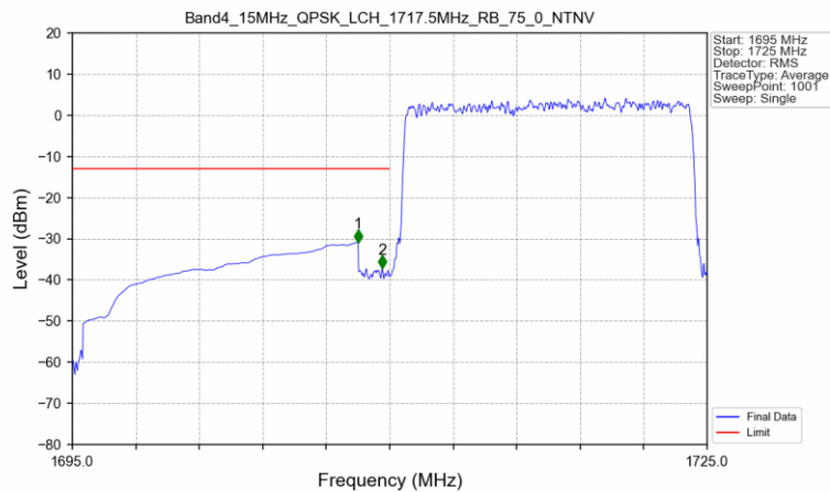
Band4_15MHz_QPSK_LCH_1717.5MHz_RB_75_0_NTNV
