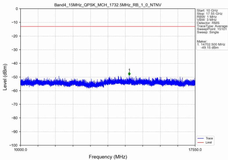
Band4_15MHz_QPSK_MCH_1732.5MHz_RB_1_0_NTNV
