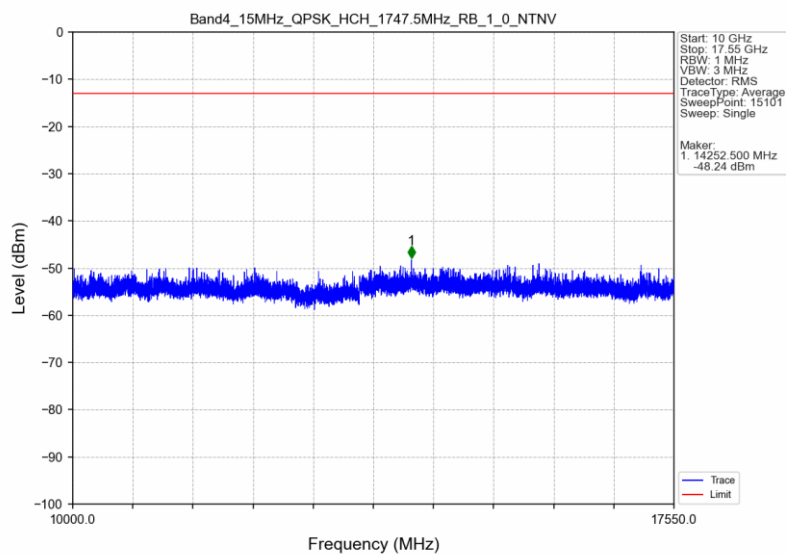
Band4_15MHz_QPSK_HCH_1747.5MHz_RB_1_0_NTNV
