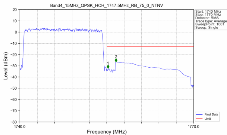
Band4_15MHz_QPSK_HCH_1747.5MHz_RB_75_0_NTV
