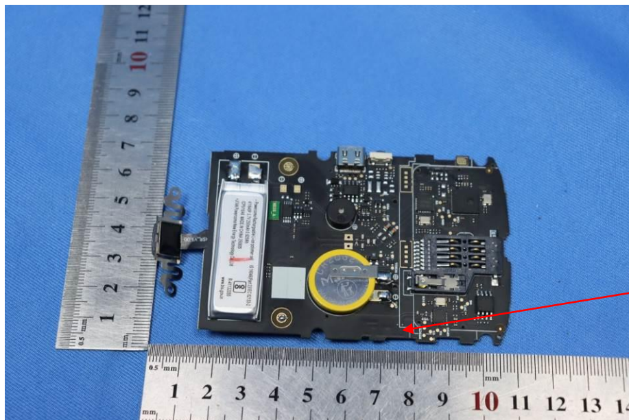
BT antenna
