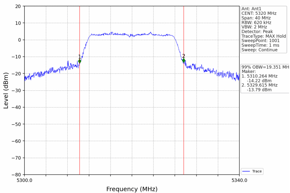
802.11a_HCH_5320MHz_Ant1_NTNV
