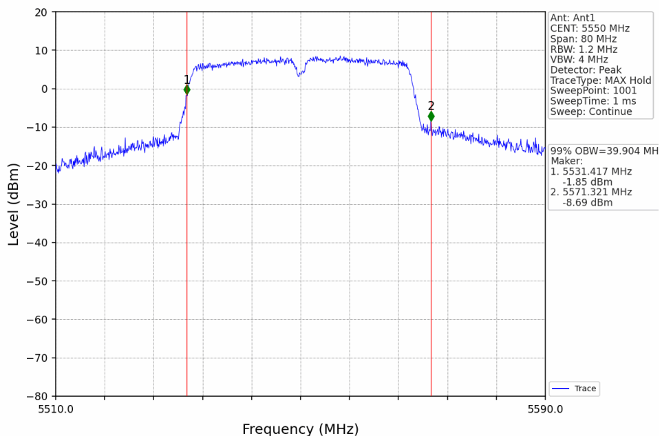
802.11n(HT40)_MCH_5550MHz_Ant1_NTNV
