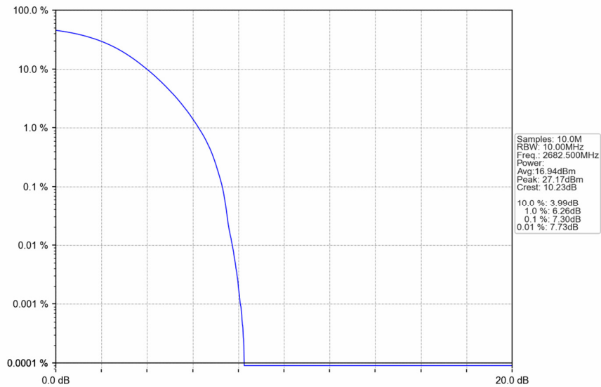
Band41 15MHz QPSK HCH 2682.5MHz RB 75 0 NTN
