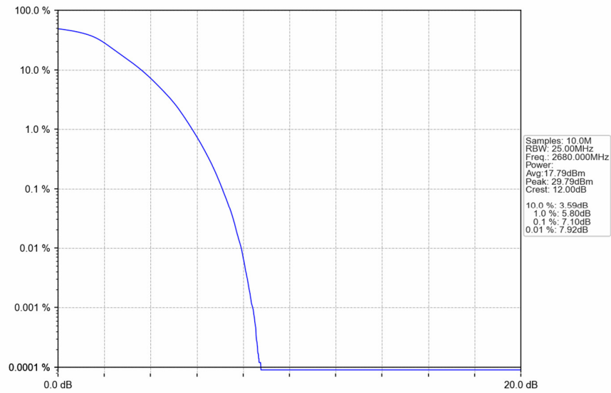
Band41 20MHz QPSK HCH 2680MHz RB 100 0 NTN
