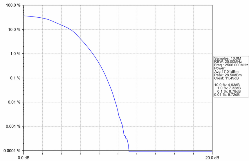
Band41 20MHz 16QAM LCH 2506MHz RB 100 0 NTN
