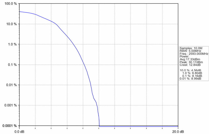
Band41 5MHz 16QAM MCH 2593MHz RB 25 0 NTNV
