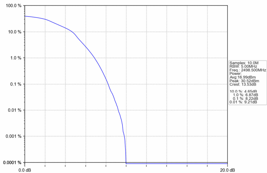
Band41 5MHz 16QAM LCH 2498.5MHz RB 25 0 NTNV
