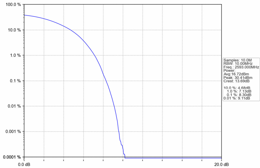
Band41 15MHz 16QAM MCH 2593MHz RB 75 0 NTNV
