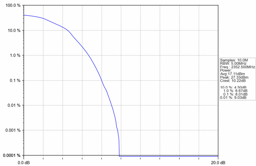
Band40b 5MHz 16QAM LCH 2352.5MHz RB 25 0 NTNV
