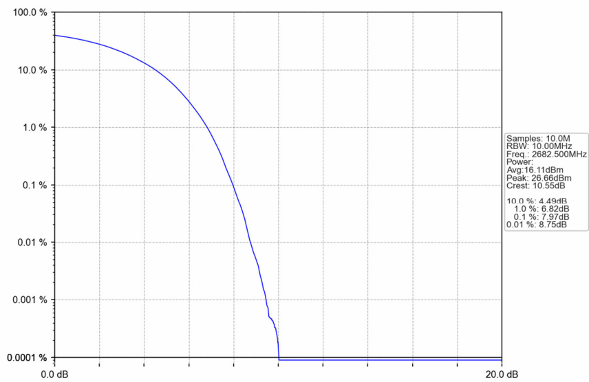
Band41 15MHz 16QAM HCH 2682.5MHz RB 75 0 NTNV
