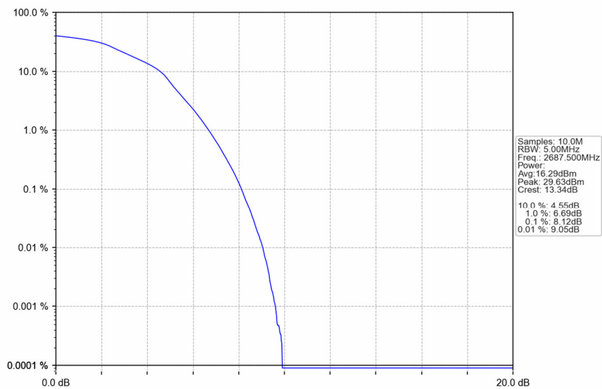
Band41 5MHz 16QAM HCH 2687.5MHz RB 25 0 NTNV
