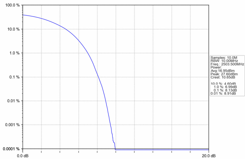
Band41 15MHz 16QAM LCH 2503.5MHz RB 75 0 NTN
