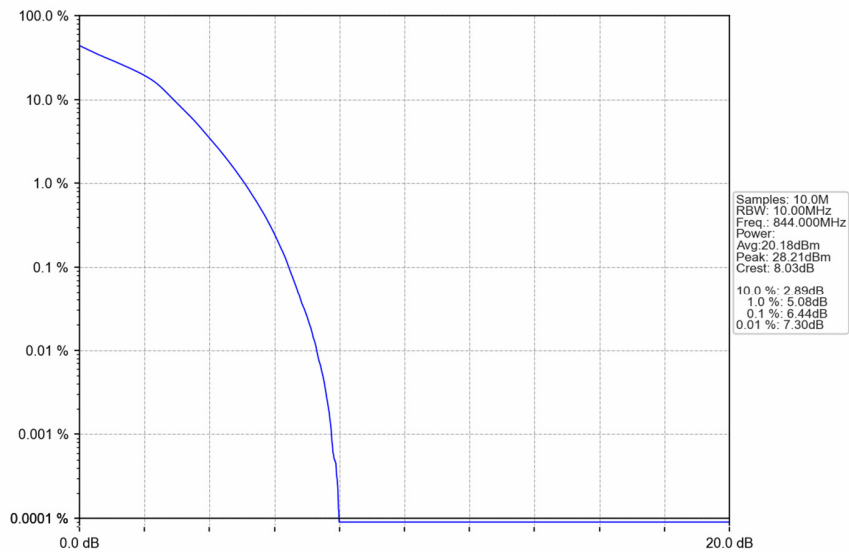
Band5 10MHz 16QAM HCH 844MHz RB 50 0 NTNV
