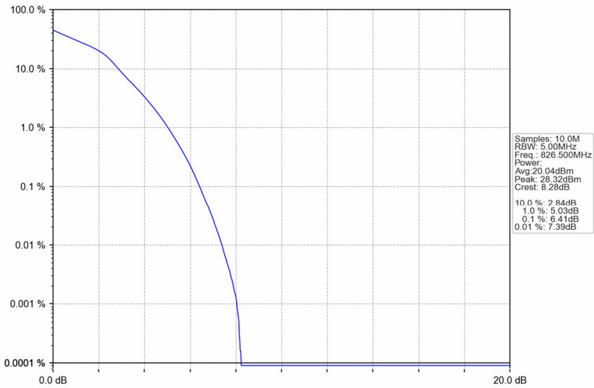
Band5 5MHz 16QAM LCH 826.5MHz RB 25 0 NTN
