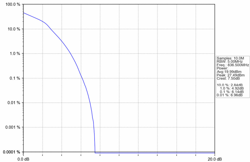
Band5 5MHz 16QAM MCH 836.5MHz RB 25 0 NTNV
