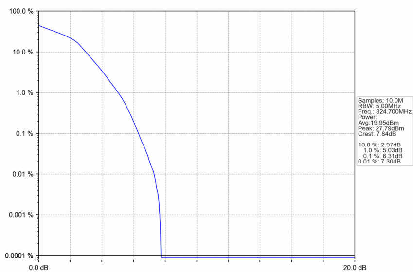
Band5 1.4MHz 16QAM LCH 824.7MHz RB 6 0 NTNV
