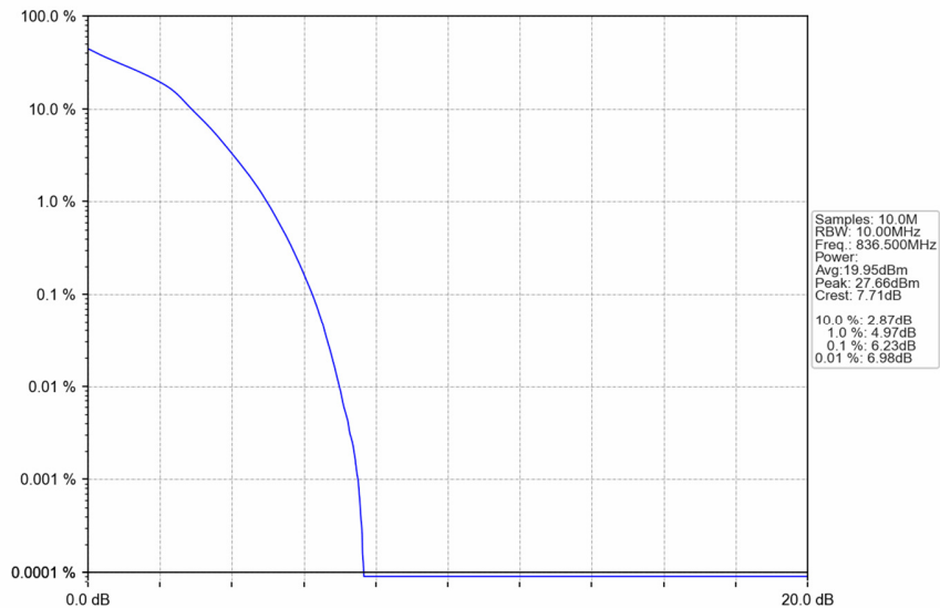
Band5 10MHz 16QAM MCH 836.5MHz RB 50 0 NTNV
