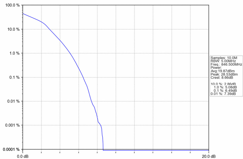
Band5 5MHz 16QAM HCH 846.5MHz RB 25 0 NTNV
