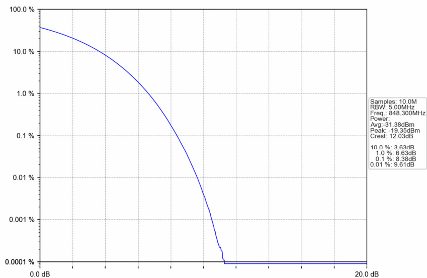
Band5 1.4MHz QPSK HCH 848.3MHz RB 6 0 NTNV
