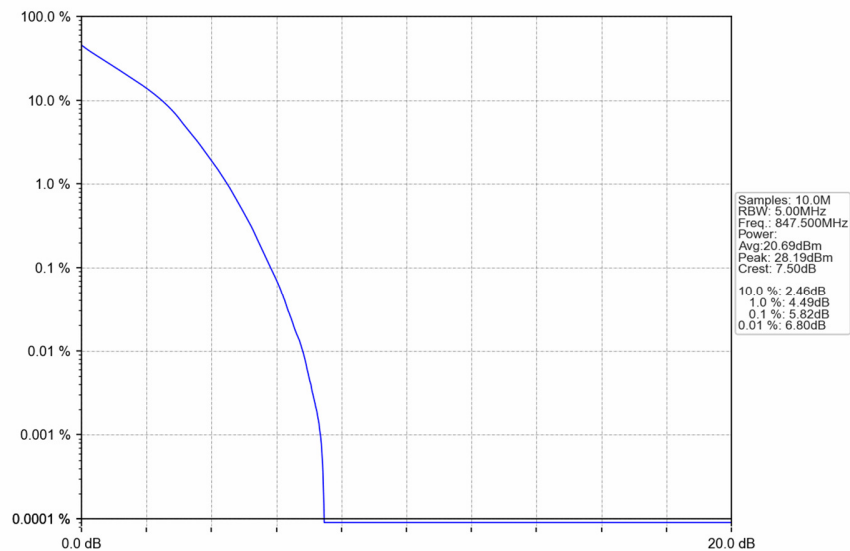
Band5 3MHz QPSK HCH 847.5MHz RB 15 0 NTN
