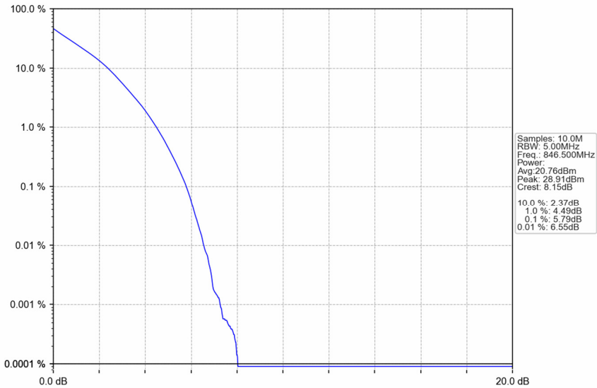
Band5 5MHz QPSK HCH 846.5MHz RB 25 0 NTN
