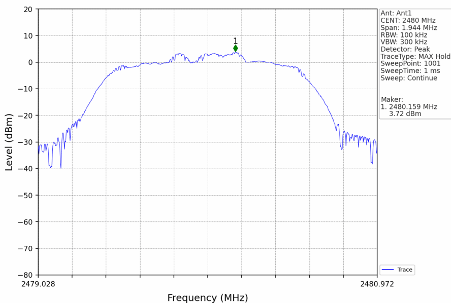
Pi/4DQPSK_2DH5_HCH_2480MHz_Ant1_NTNV
