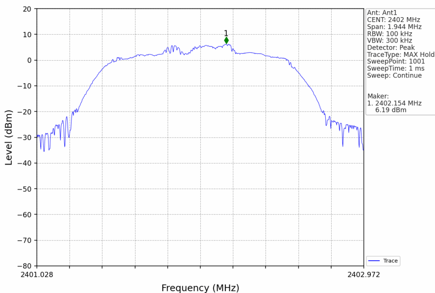
Pi/4DQPSK_2DH5_LCH_2402MHz_Ant1_NTNV
