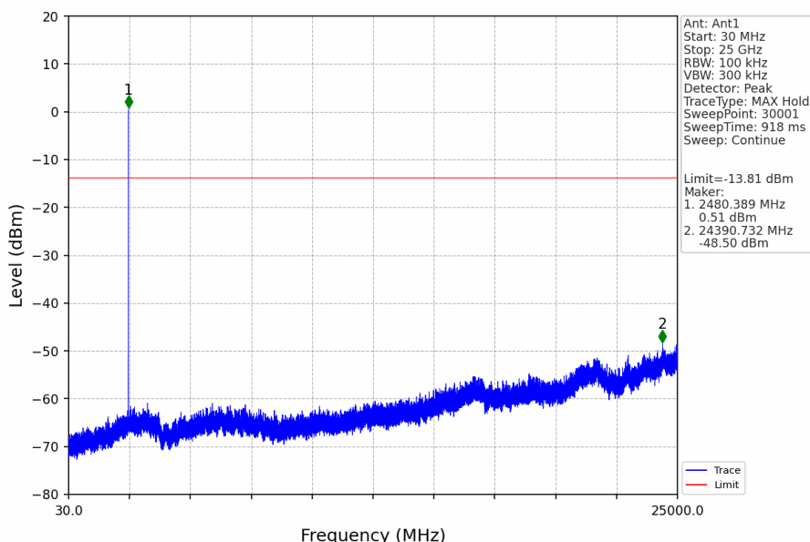
Pi/4DQPSK_2DH5_HCH_2480MHz_Ant1_NTNV
