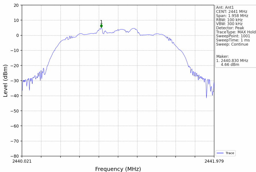
8DPSK_3DH5_MCH_2441MHz_Ant1_NTNV
