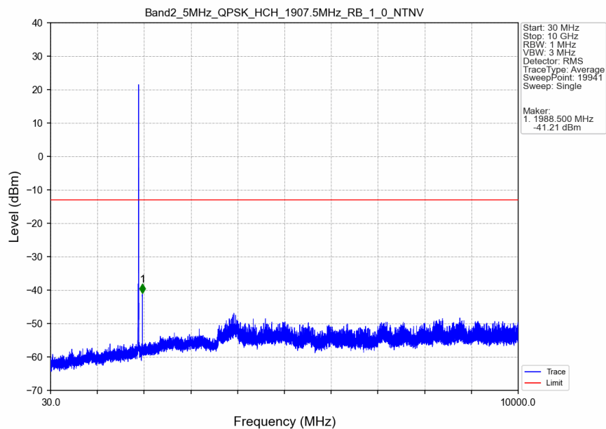
Band2_5MHz_QPSK_HCH_1907.5MHz_RB_1_0_NTNV
