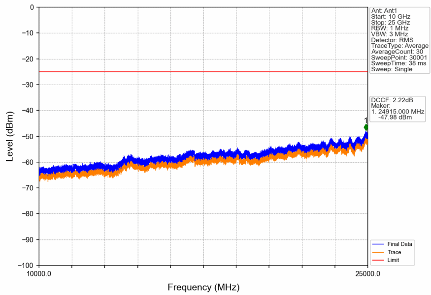
Band38_10MHz_16QAM_HCH_2615MHz_RB_1_0_NTNV
