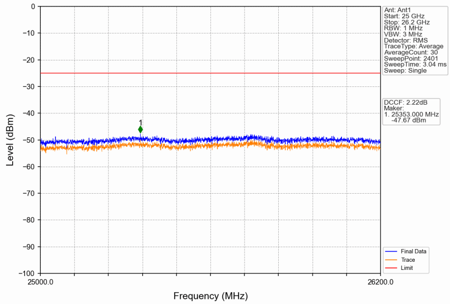
Band38_5MHz_16QAM_HCH_2617.5MHz_RB_1_0_NTNV
