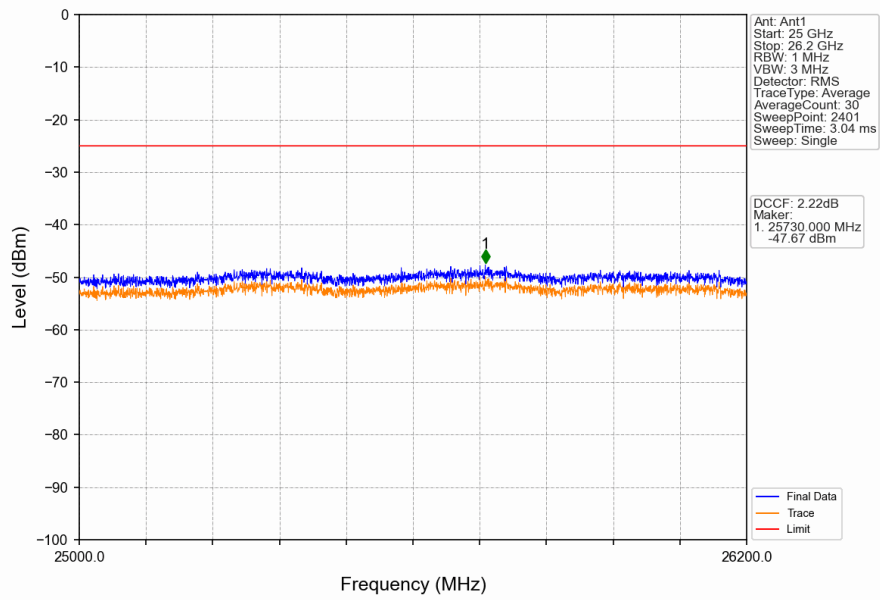
Band38_10MHz_16QAM_HCH_2615MHz_RB_1_0_NTNV
