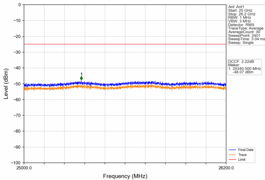
Band38_10MHz_16QAM_HCH_2615MHz_RB_1_0_NTNV
