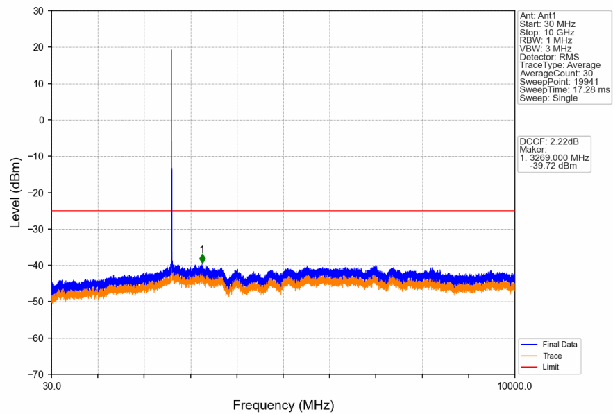
Band38_10MHz_16QAM_HCH_2615MHz_RB_1_0_NTNV
