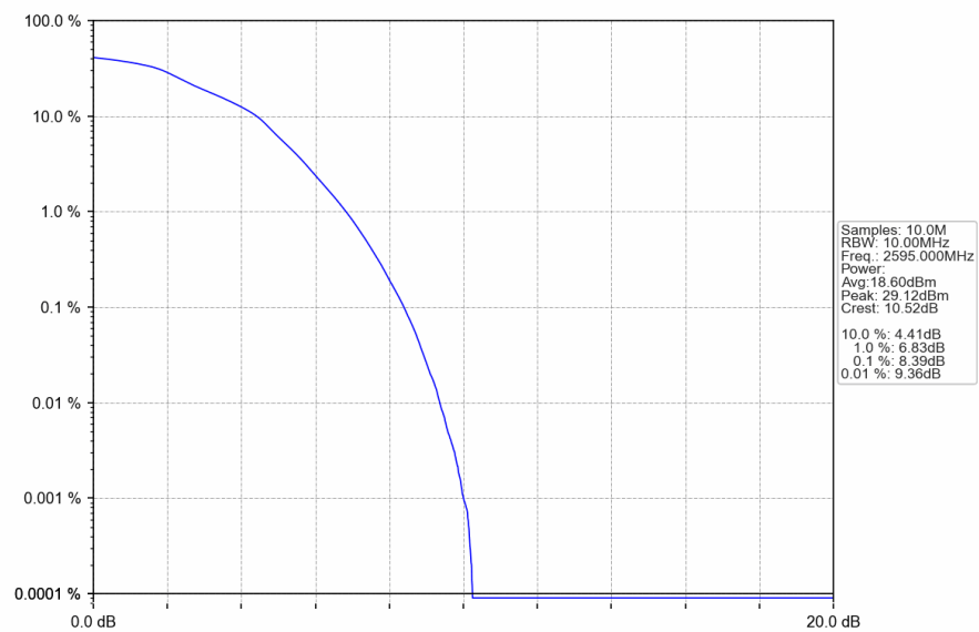
Band38 10MHz 16QAM MCH 2595MHz RB 50 0 NTNV
