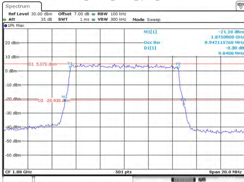
Band 2_10 MHz_Middle_QPSK_RB50#0
