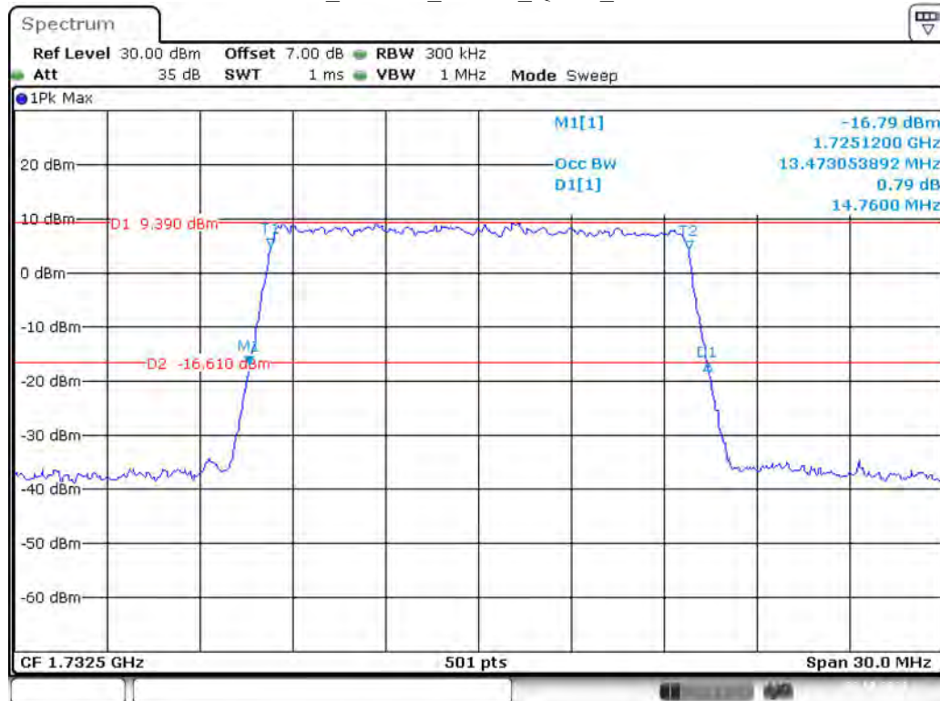
Band 4_15 MHz_Middle_QPSK_RB75#0
