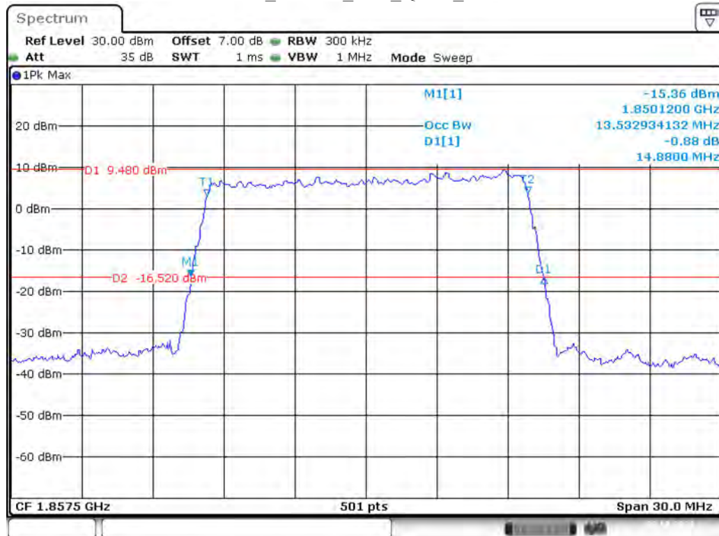
Band 25_15 MHz_Low_QPSK_RB75#0
