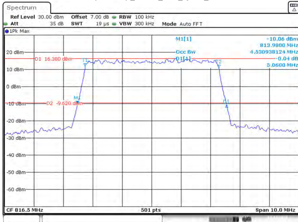
Band 26(Part 90S)_5 MHz_Low_QPSK_RB25#0
