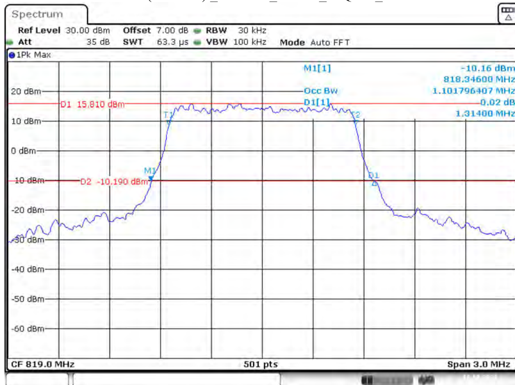
Band 26(Part 90S) _1.4 MHz_Middle_16QAM_RB6#0
