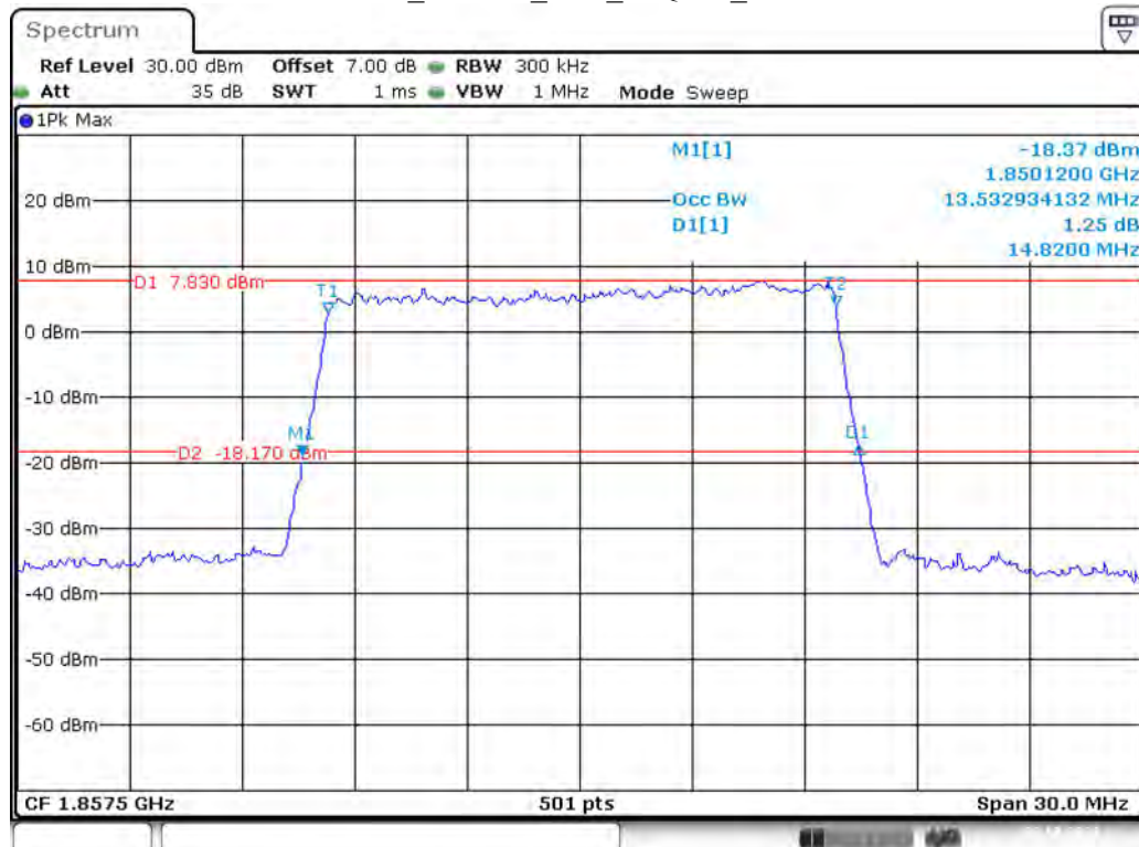
Band 25_15 MHz_Low_16QAM_RB75#0
