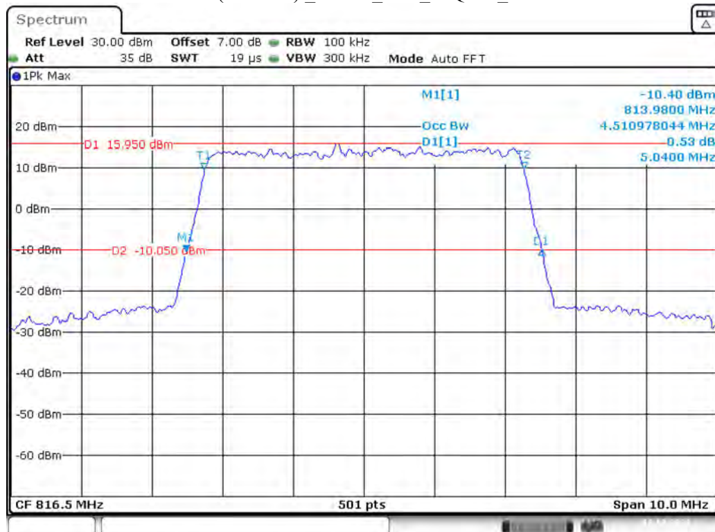
Band 26(Part 90S)_5 MHz_Low_16QAM_RB25#0
