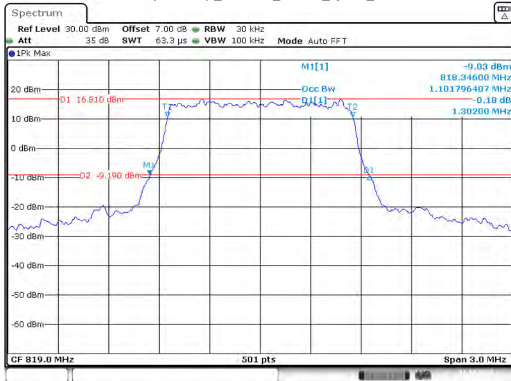
Band 26(Part 90S) _1.4 MHz_Middle_QPSK_RB6#0
