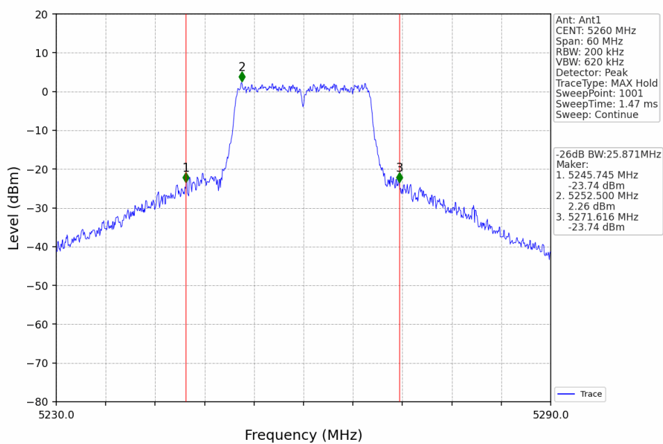
802.11a_LCH_5260MHz_Ant1_NTNV
