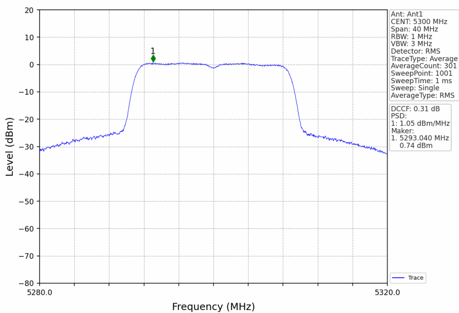
802.11n(HT20)_MCH_5300MHz_Ant1_NTNV
