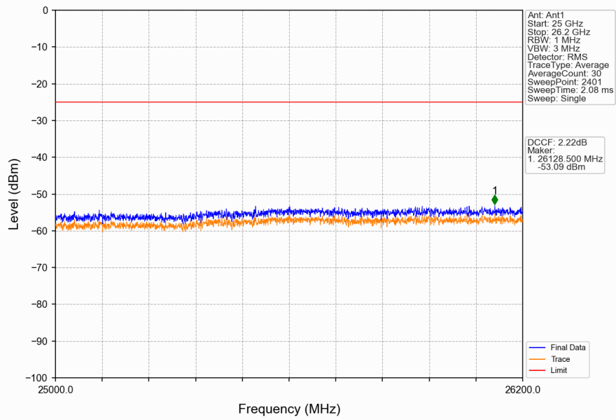
Band38_5MHz_16QAM_HCH_2617.5MHz_RB_1_0_NTNV
