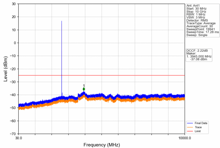
Band38_5MHz_16QAM_HCH_2617.5MHz_RB_1_0_NTNV
