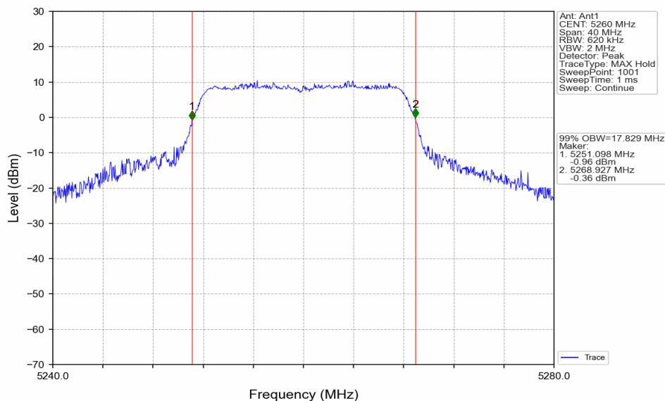
802.11a_LCH_5260MHz_Ant1_NTNV
