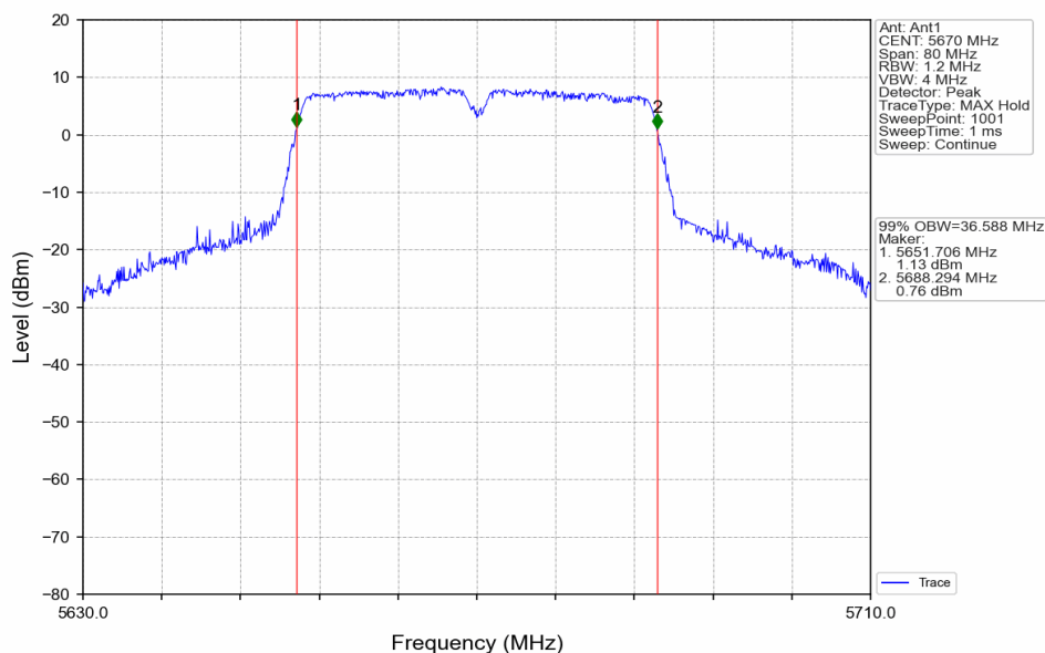
802.11ac(VHT40)_HCH_5670MHz_Ant1_NTNV
