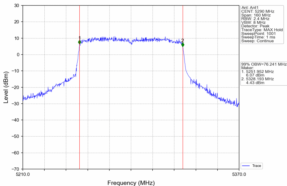
802.11ac(VHT80)_MCH_5290MHz_Ant1_NTNV
