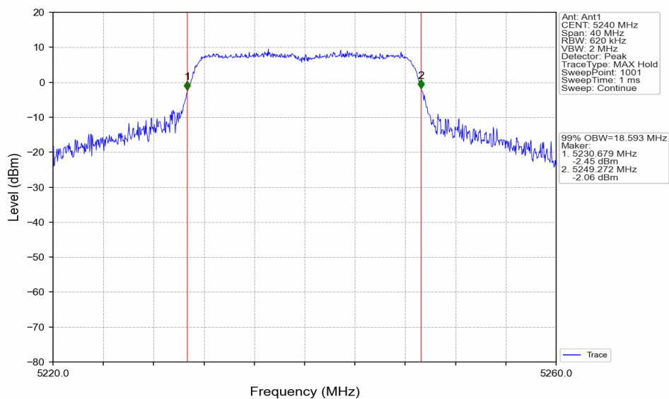
802.11ac(VHT20)_HCH_5240MHz_Ant1_NTNV
