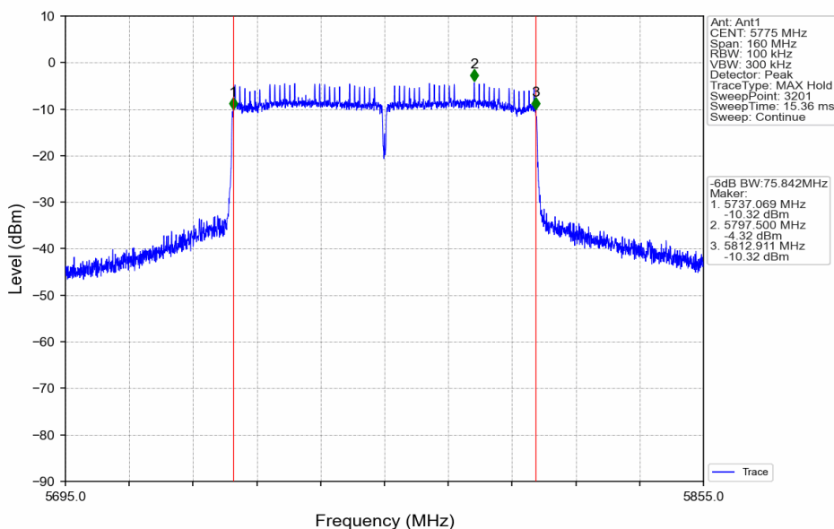
802.11ac(VHT80)_MCH_5775MHz_Ant1_NTNV
