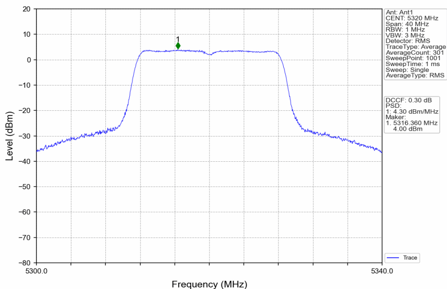
802.11a_HCH_5320MHz_Ant1_NTNV
