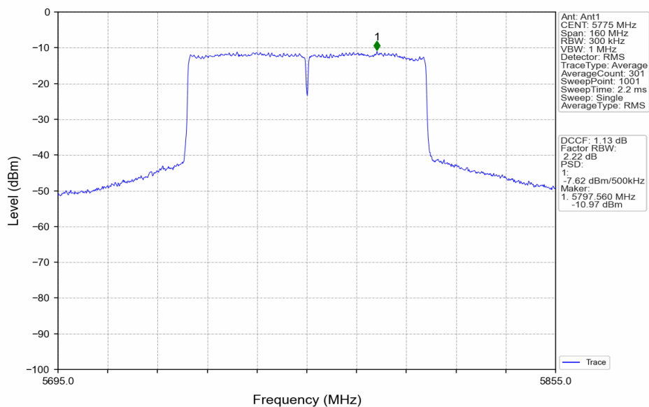
802.11ac(VHT80)_MCH_5775MHz_Ant1_NTNV
