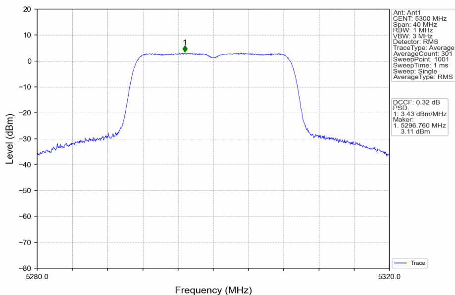
802.11ac(VHT20)_MCH_5300MHz_Ant1_NTNV
