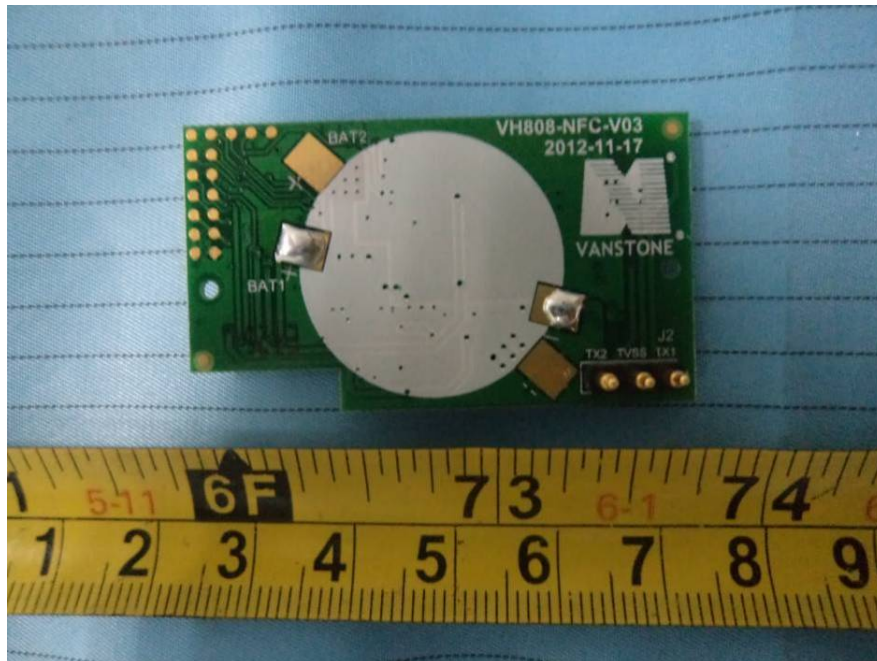
EUT – NFC Board Bottom View 2
