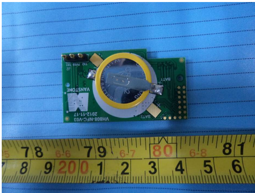
EUT – NFC Board Bottom View 1
