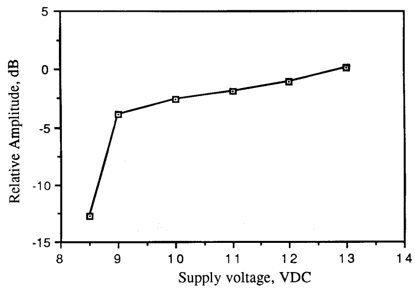
Figure 6.4. Relative emission at 300.0 MHz vs. supply voltage. (pulsed emission)
