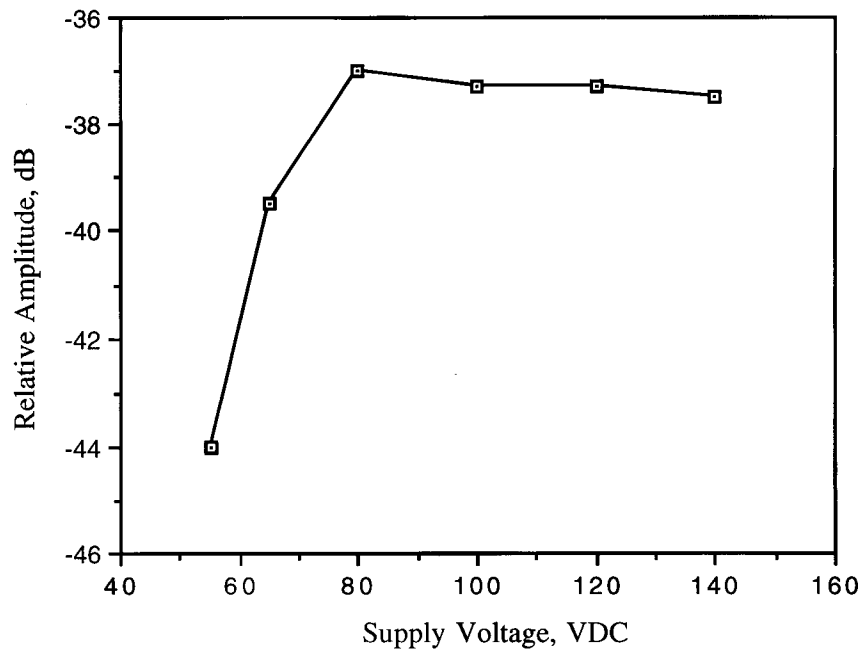
Figure 6.2. Relative emission at "fundamental" vs. supply voltage.
