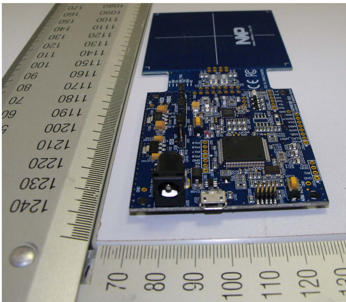
Figure 3: Side view
