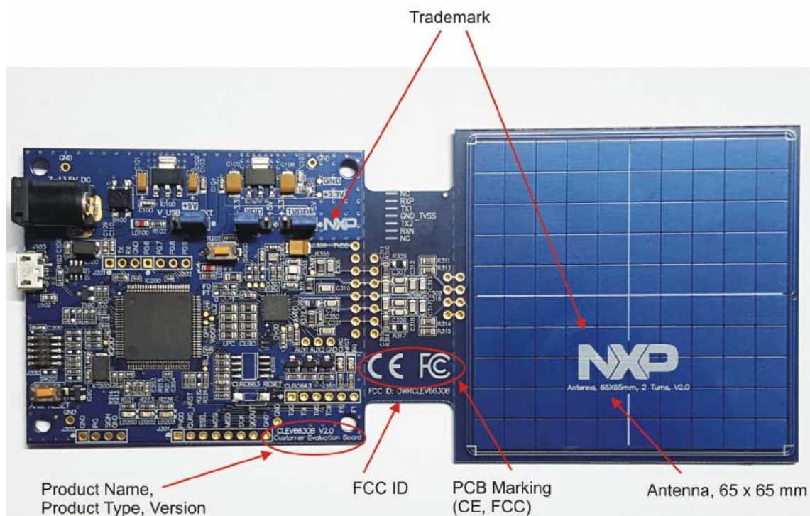
Figure 4: Label location
