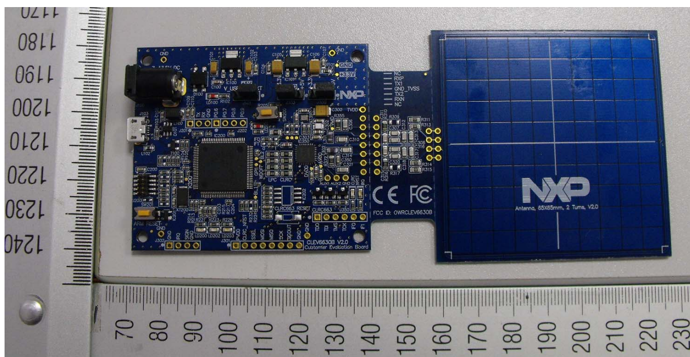
Figure 2: Top side
