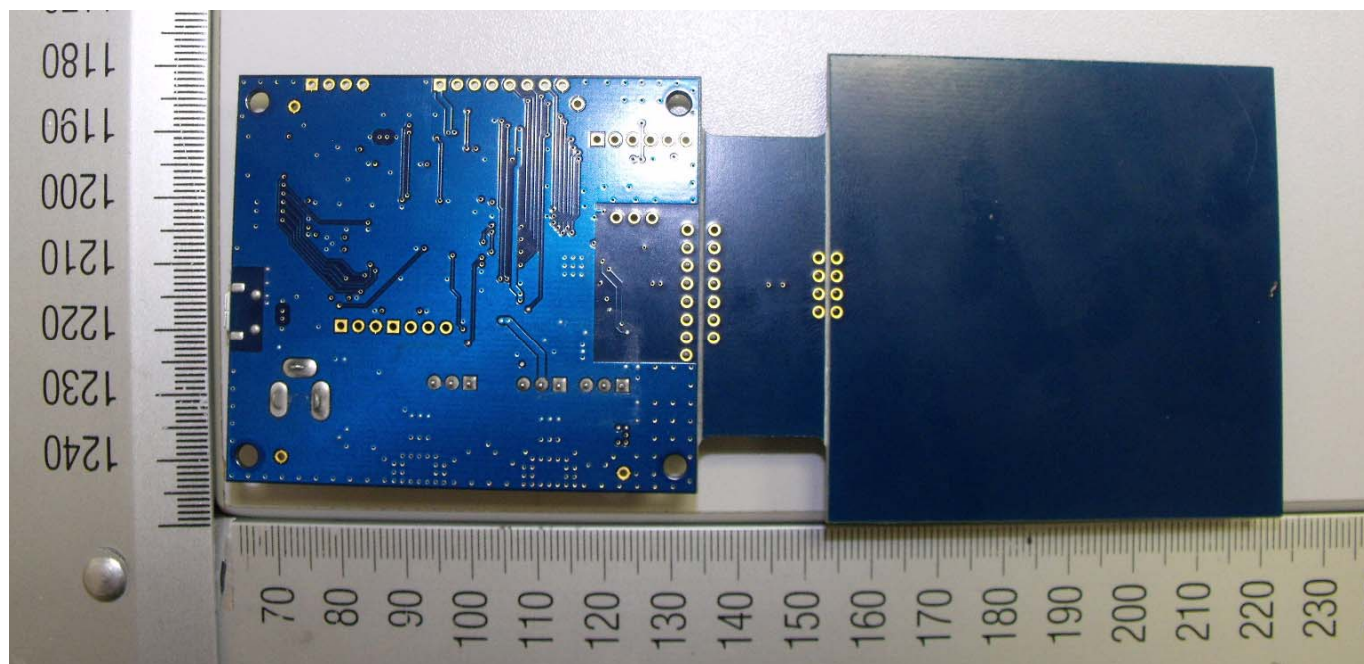
Figure 1: Bottom side
