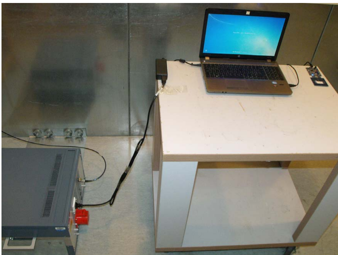
Figure 2: Conducted emission test
