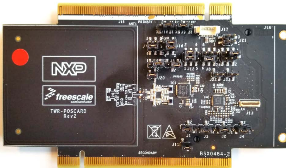
Fig 2. TWR-POSCARD V2 Top view
