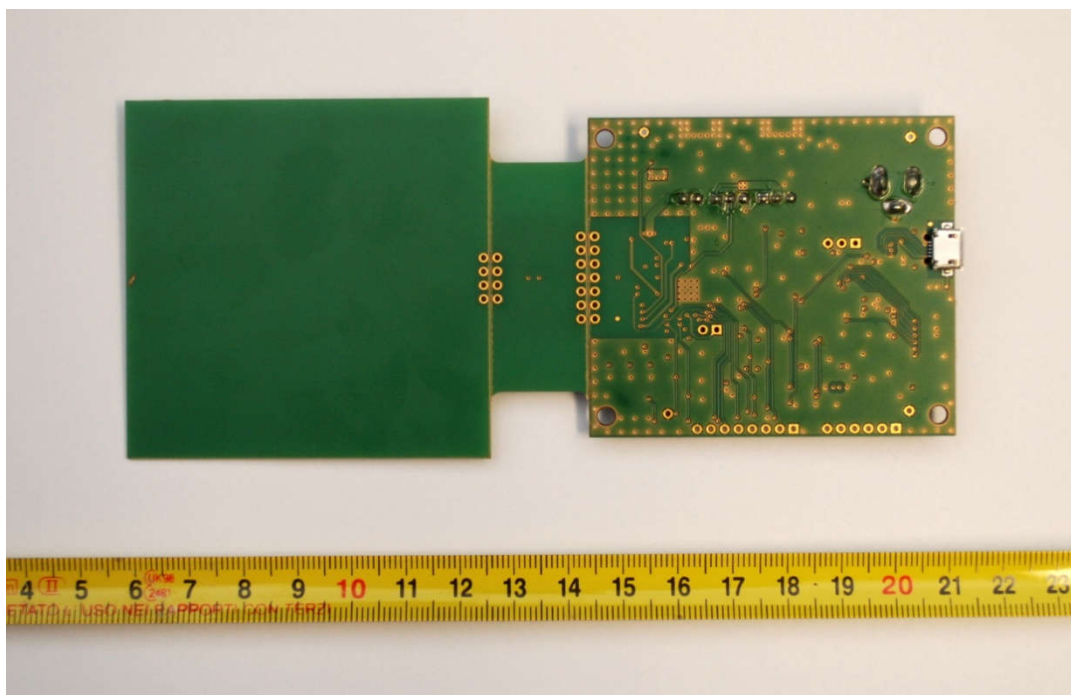
Picture 2: Customer Development Board PNEV5180B - bottom view.
