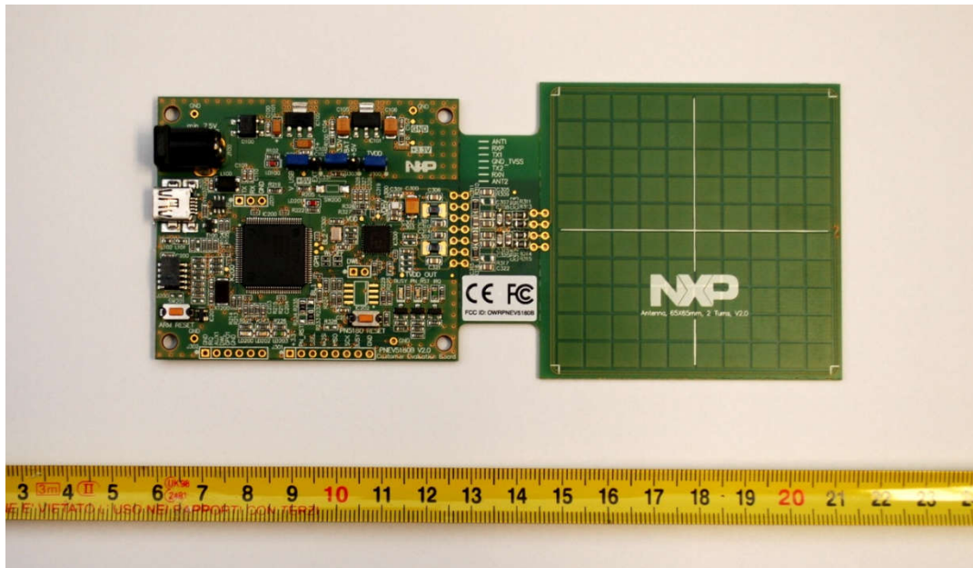
Picture 1: Customer Development Board PNEV5180B - top view.
