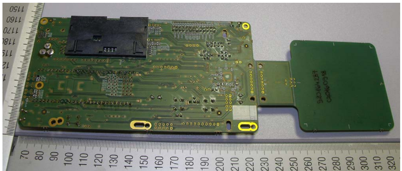
Figure 2: Bottom view
