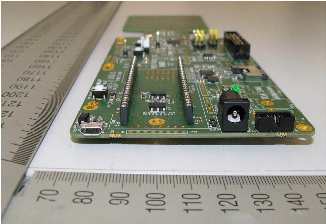
Figure 3: Side view
