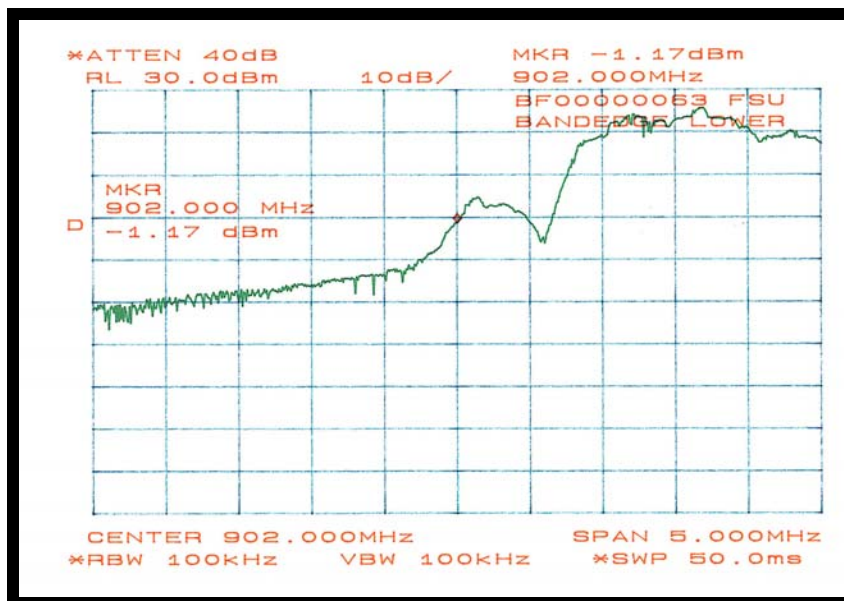
Figure 19: Plot of Lower Band-Edge Measurement at 902MHz
