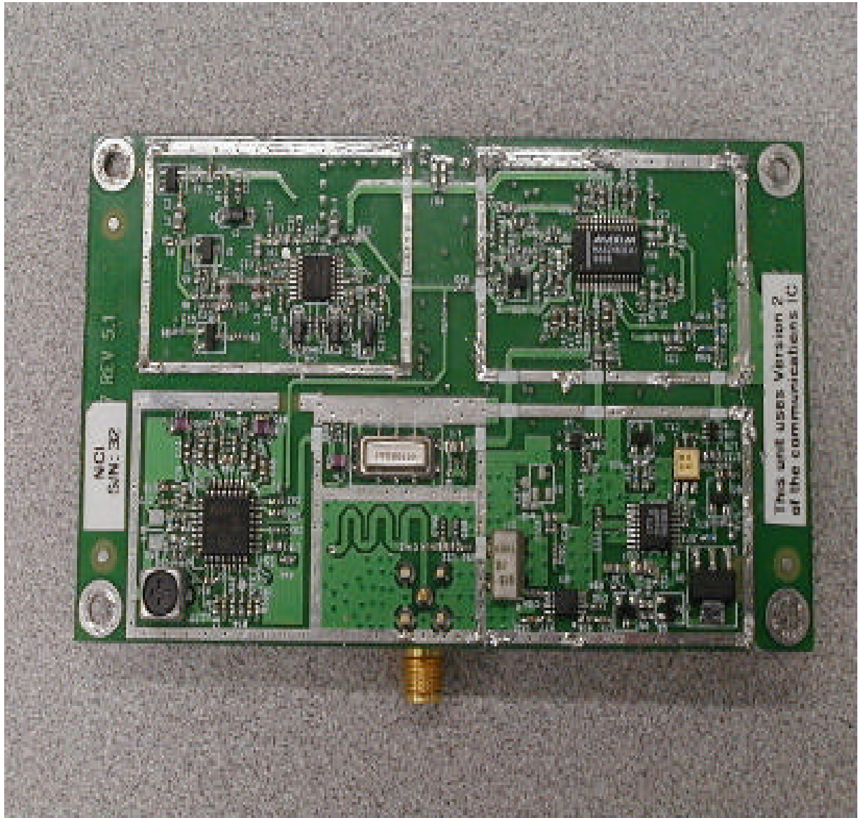
Rear View Transceiver Board without Shield
