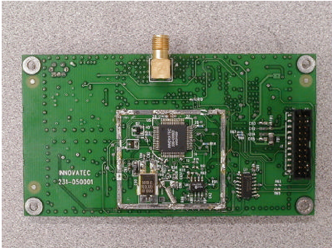
Front View Transceiver Board without Shield
