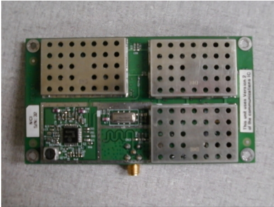
Front View of Transceiver Board
