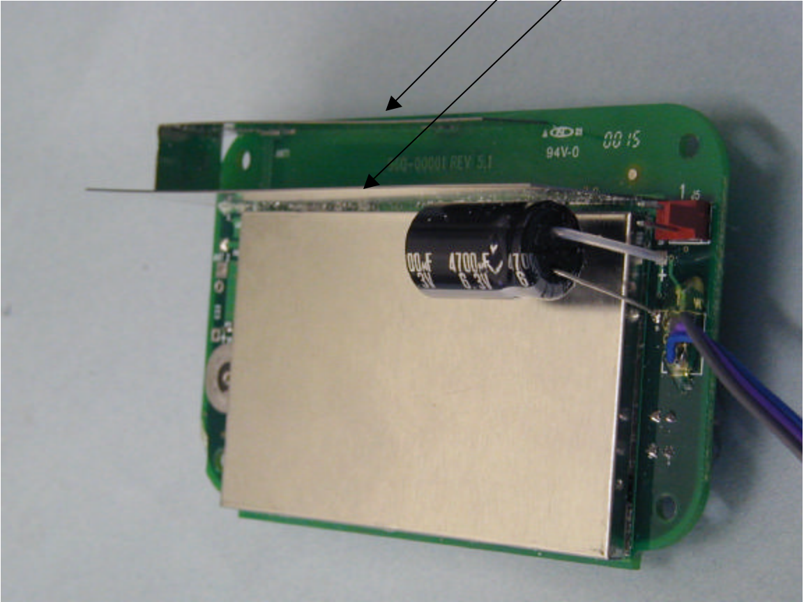
Antenna View #2
