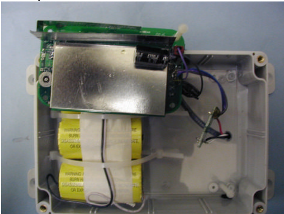
Internal Layout without Enclosure— Rear View
