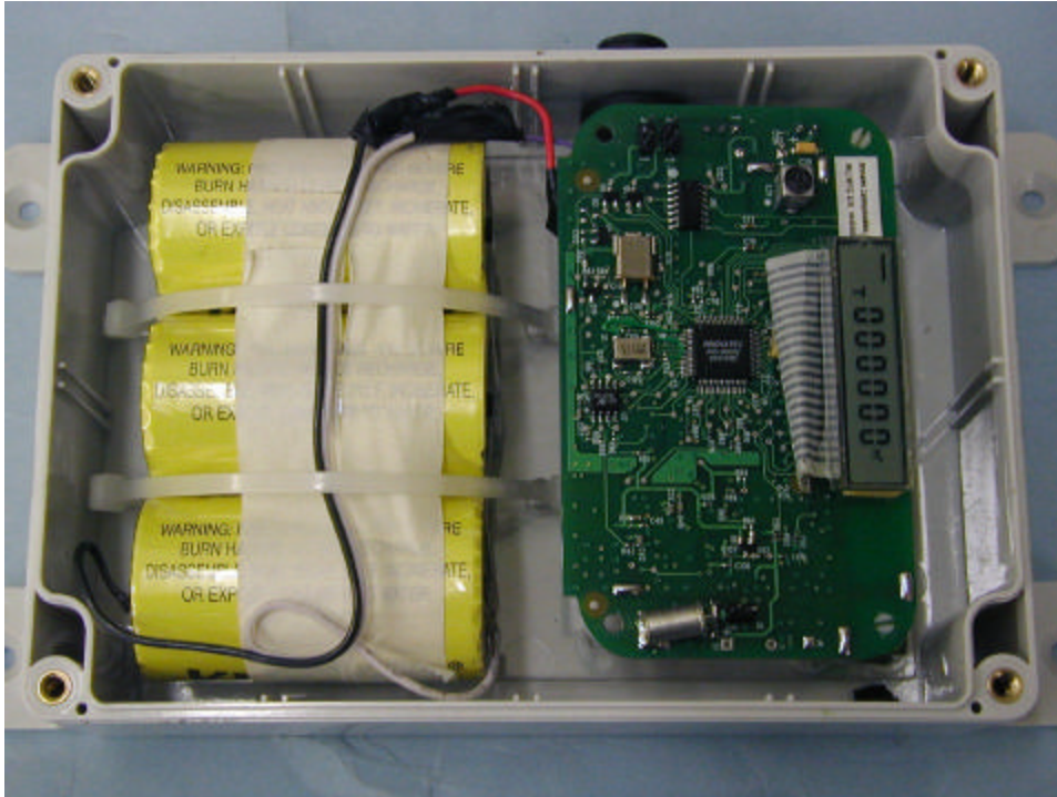
Internal Layout without Enclosure— Front View
